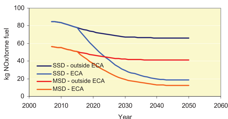
Figure 7.5 Future NO x emission factors (3% fleet growth per year, year vessel life)
