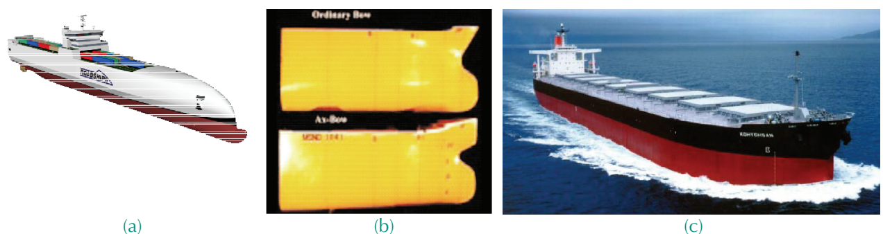
Figure A2.2 (a) Example of a superslender monohull with outriggers (copyright STX Europe, 2008); (b) Axe-bow design; and (c) 172,000 DWT Capesize bulk carrier Kohyohsan, built with an axe bow for Mitsui O.S.K. Lines, Ltd in 2001.
