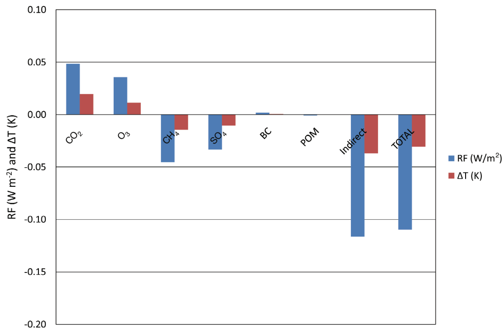
Figure 8.4 Global mean radiative forcings ( W\ m^{-2} ) and temperature responses (K) in 2007 from shipping emissions. The figure does not include the positive RF that could possibly occur from the interaction of BC with snow, which has so far not been investigated for ships.
