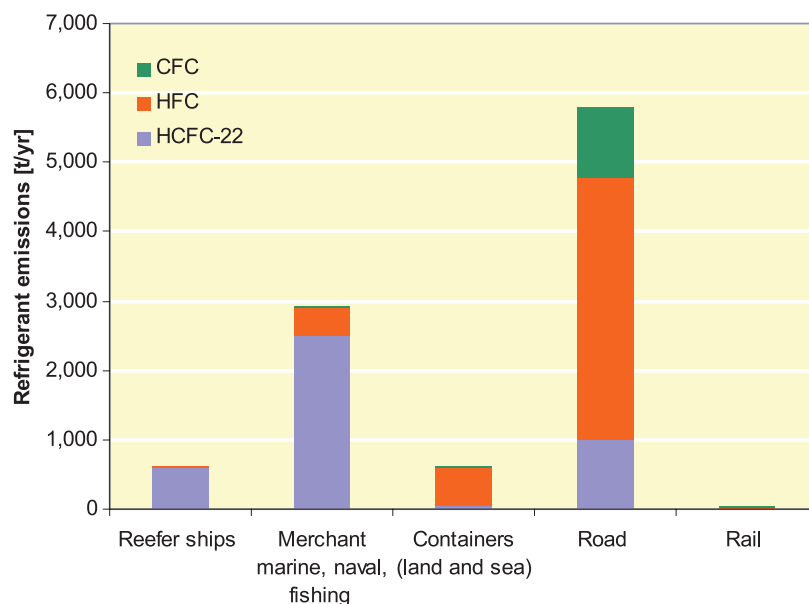
Figure 3.4 Emissions of refrigerants from transport in 2003, UNEP [33]
