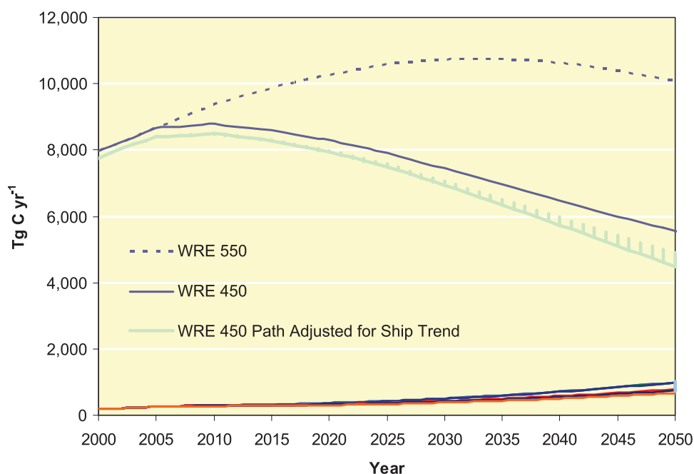
Figure 8.7 Comparison of modelled shipping emissions, curves for WRE 450 and WRE 550, and WRE 450 adjusted for ship emissions (global total minus the emissions arising from shipping)
