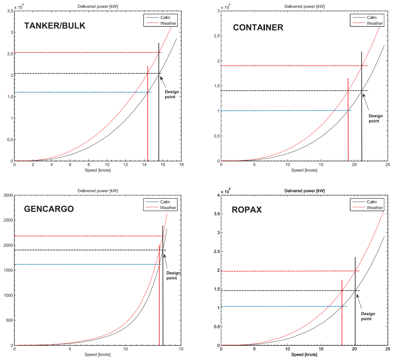
Figure A3.3 Speed loss (drop) at constant delivered power P_D or at increased delivered power P_D , at constant speed, of the advance of vessels in head weather conditions (irregular waves and wind from the same direction 180^\circ ) for four different types of ships, according to MARINTEK's 2008 direct model tests database, with the assumption of Beaufort number BN ( Bft ) = 6 for Tanker/Bulk, BN ( Bft ) = 6 for Container, BN ( Bft ) = 3 for GenCargo, BN ( Bft ) = 6 for RoPax
