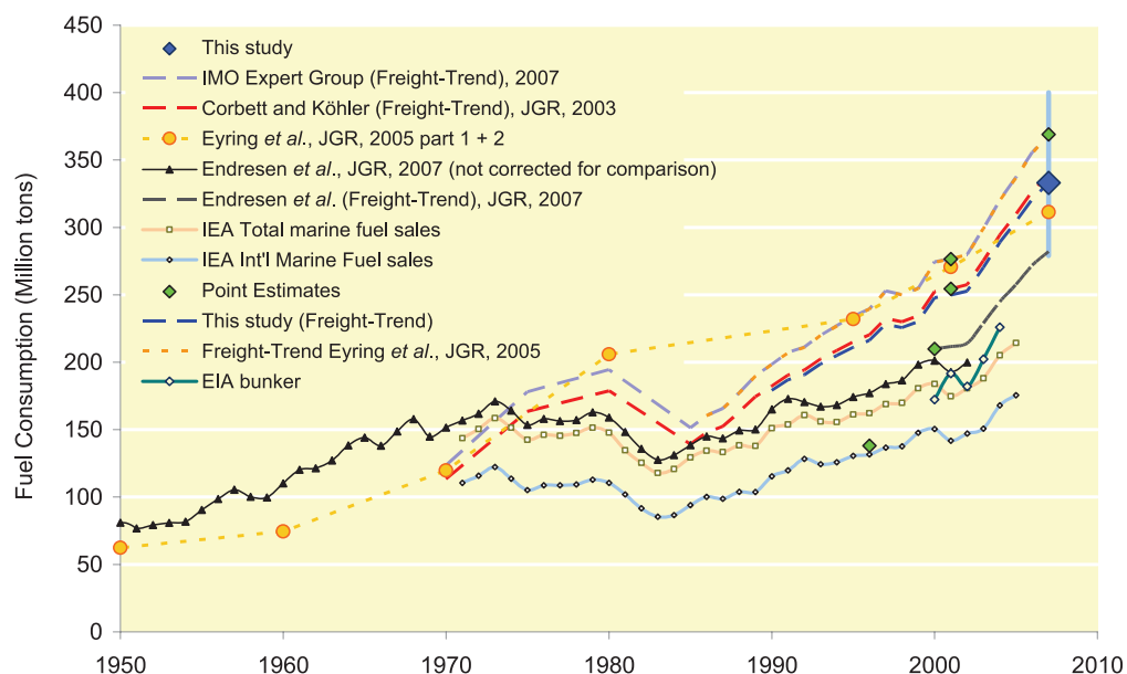
Figure 3.2 World fleet fuel consumption (except military vessels) from different activity-based estimates and statistics. Symbols indicate the original estimates for individual years and the solid lines show the original estimates of trend. Dashed lines show the backcast and forecast, calculated from the time evolution of freight tonne-miles with the point estimates. The blue square shows the activity-based estimate from this study and the blue range bar indicates the high and low bound estimates
