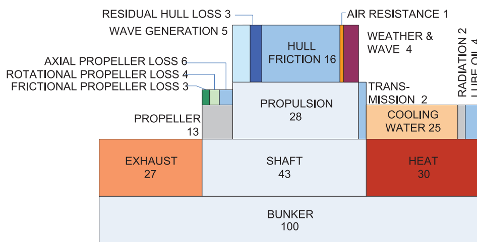
Figure A2.1 Use of propulsion energy on board a small cargo ship, head sea, Beaufort 6
