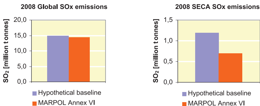
Figure 4.4 Reductions of emissions of SO x estimated for 2008
