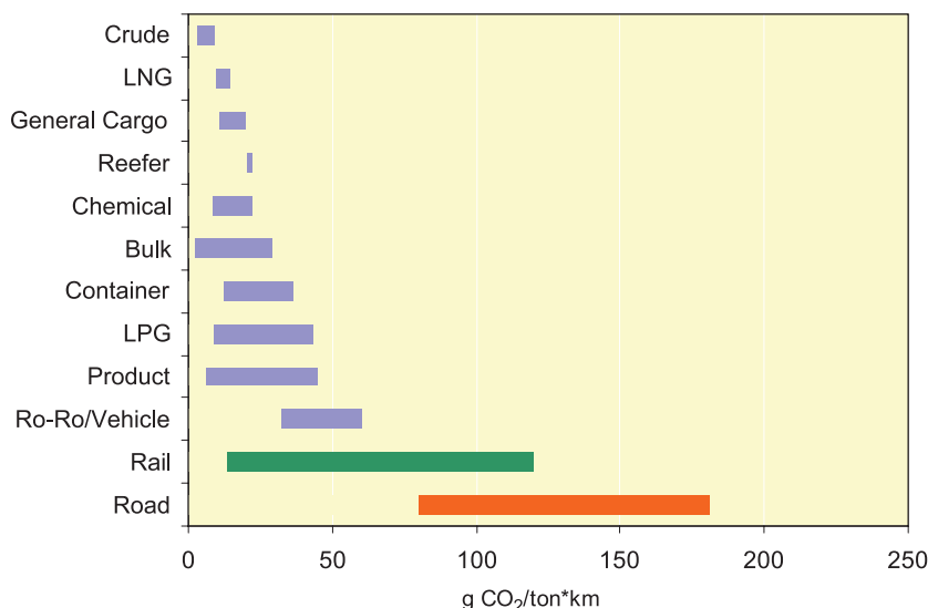
Figure 9.2 Typical range of ship CO 2 efficiencies compared to rail and road
