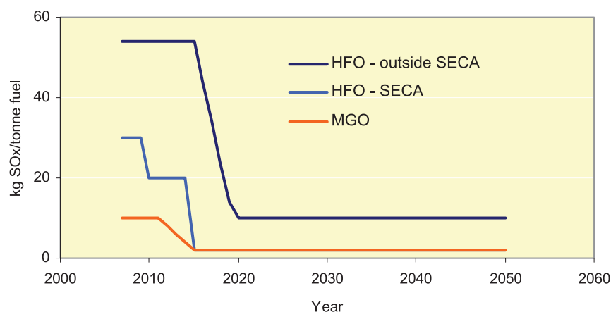
Figure 7.6 Future SO x emission factors used in scenarios. The future limit of 3.50% in 2012 on global sulphur content is not expected to influence the average emission factor
