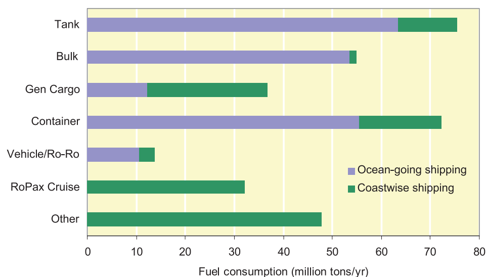
Figure A1.7 Fuel consumption (million tonnes) by main ship categories, showing assumed typical types of operation (Coastwise shipping is mainly ships < 15,000 dwt, RoPax, Cruise, Service and Fishing)
