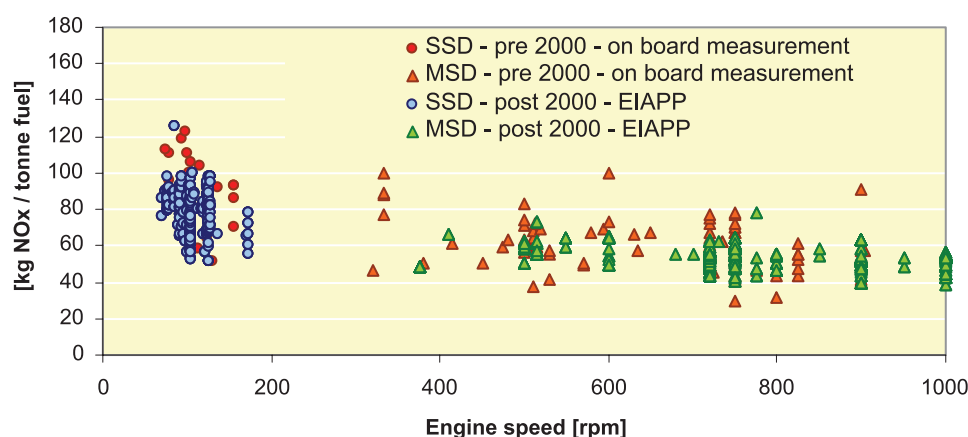
Figure 4.2 NO x emission factors from measurement and from EIAPP certificates
