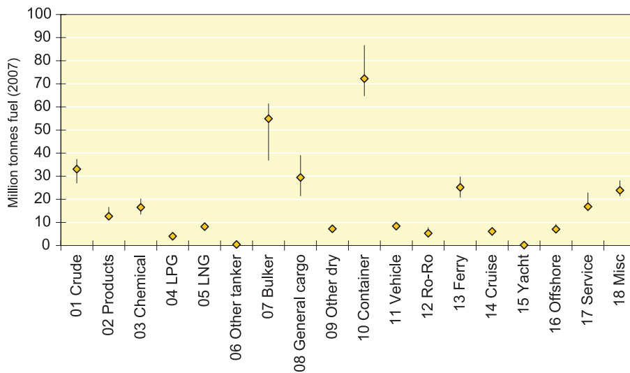
Figure A1.6 Estimated fuel consumption (million tonnes) in 2007 by main ship categories, with uncertainty bars
