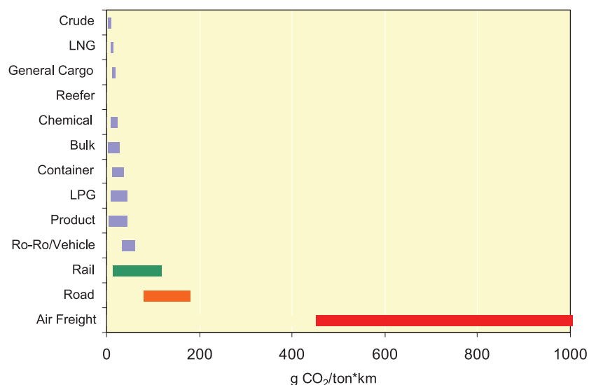
Figure 9.3 Typical range of ship CO 2 efficiencies compared to rail, road and air freight
