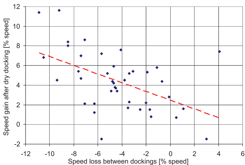
Figure A2.5 The effect of dry-docking on the speed of a tank ship; the analysis is based on data reported by the ship (primarily, TBT-based self-polishing coatings were used)
