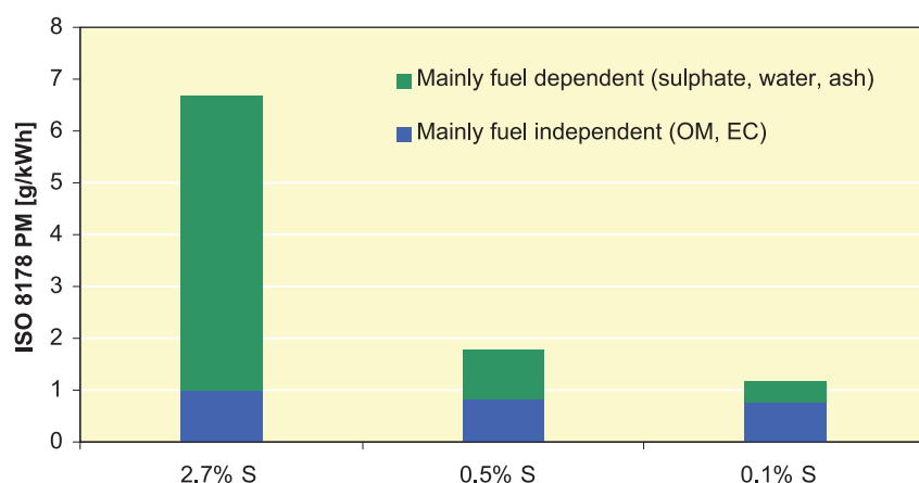
Figure A2.8 The influence of fuel on PM mass. Data: GL [7]
