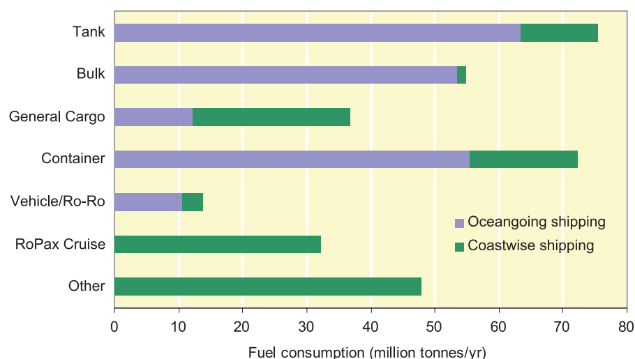
Figure 3.3 Fuel consumption, separated into consumption by main categories of vessel and assumed typical types of operation (Coastwise shipping is mainly ships < 15,000 dwt, RoPax, Cruise, Service and Fishing)
