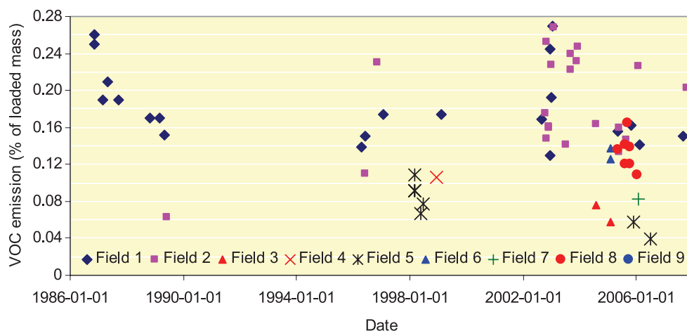
Figure 3.5 VOC emission factor measured during offshore loading in the North Sea
