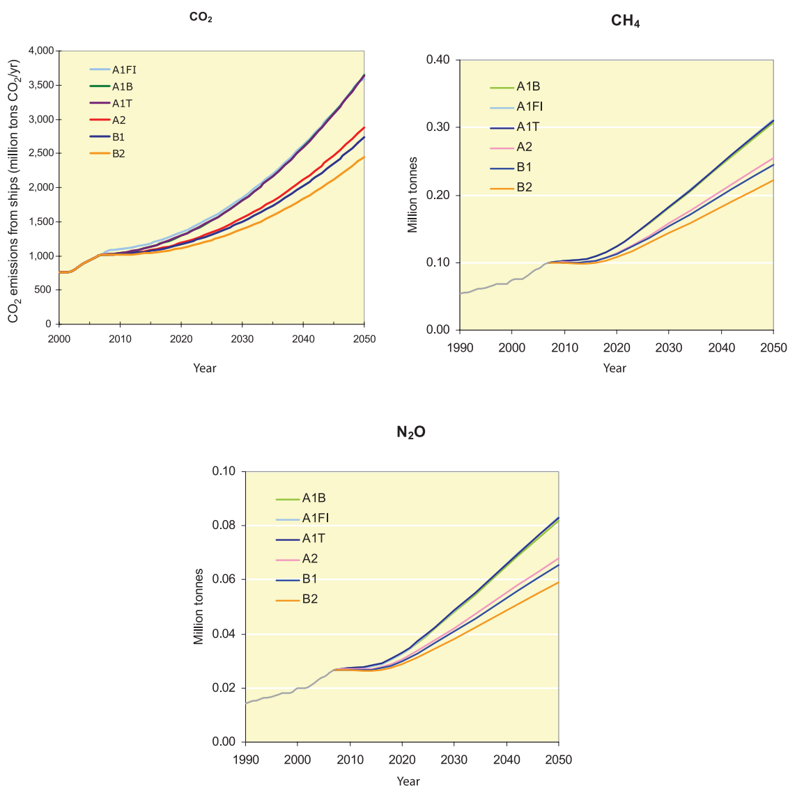
Figure 7.9 Emission scenario trajectories for GHG emissions – total shipping (exhaust emissions only)
