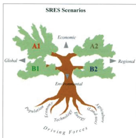
Figure 7.1 IPCC Storylines (IPCC).
