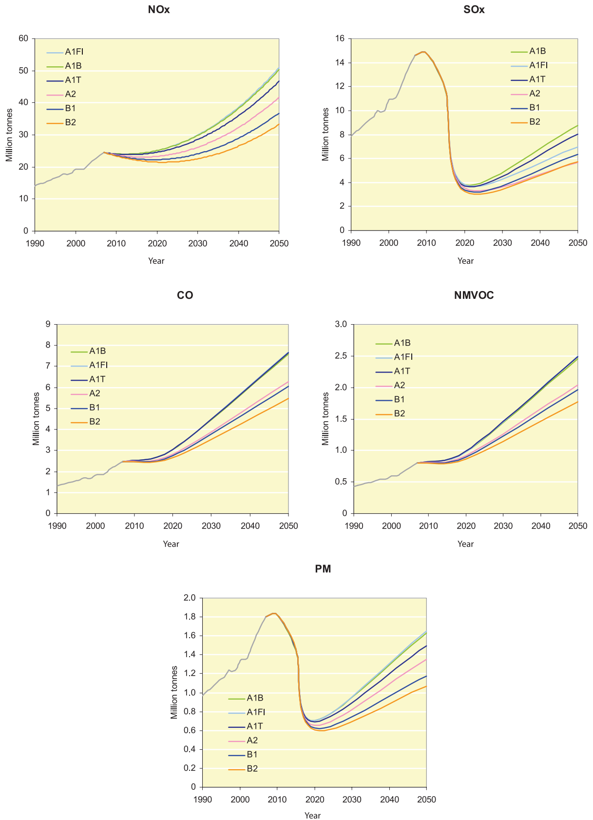
Figure 7.10 Emission scenario trajectories for other relevant substances – total shipping (exhaust emissions only)
