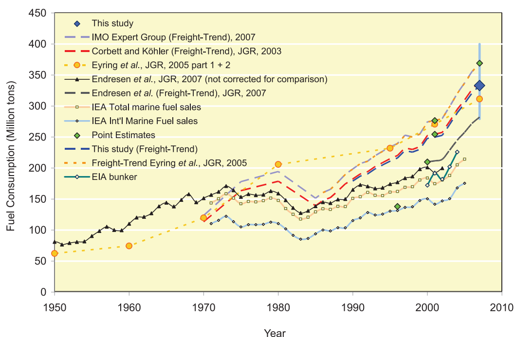
Figure A1.4 World fleet fuel consumption (except naval vessels) from different activity-based estimates and statistics. Symbols indicate the original estimates for individual years and the solid lines show the original estimates of trend. Dashed lines show the backcast and forecast, calculated from the time evolution of freight tonne-miles with the point estimates. The blue square shows the activity-based estimate from this study and the blue range bar indicates the high and low bound estimates
