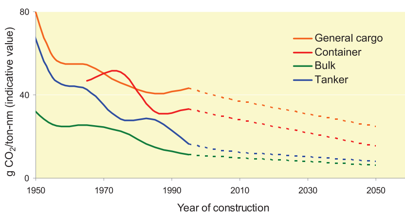
Figure 7.4 Baseline improvements in efficiency and indicated historic improvements
