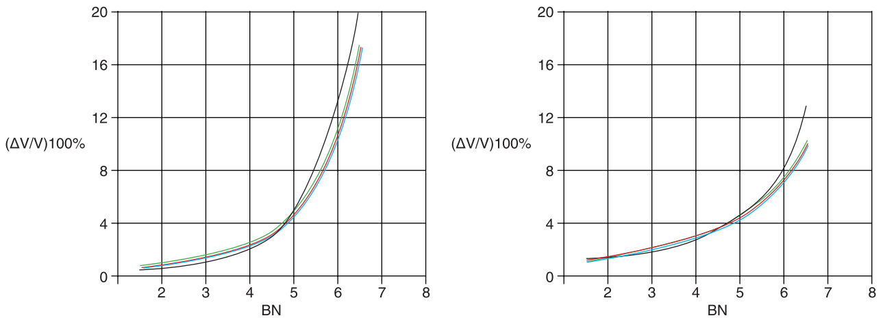
Figure A3.2 Speed loss (drop) of a ship in irregular head waves and wind (waves and wind from the same direction 180^\circ ) – comparison between the approximate formulae and detailed calculations for (a) Large tanker (loaded and/or normal condition), displacement volume \nabla = 350,000 \text{ m}^3 , Fn = 0.15 , C_B = 0.84 , L_{pp} = 336.0 \text{ m} ; (b) Large container ship (loaded and/or normal condition), displacement volume \nabla = 60,200 \text{ m}^3 , Fn = 0.25 , C_B = 0.62
