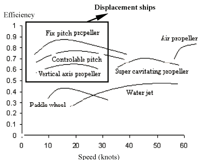
Figure A2.6 Efficiency of propulsive devices [31]
