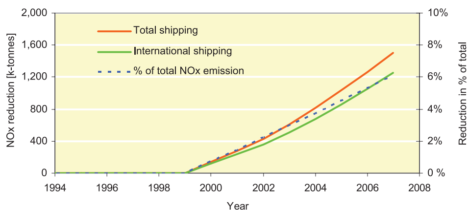
Figure 4.3 NO x reductions achieved by regulation 13
