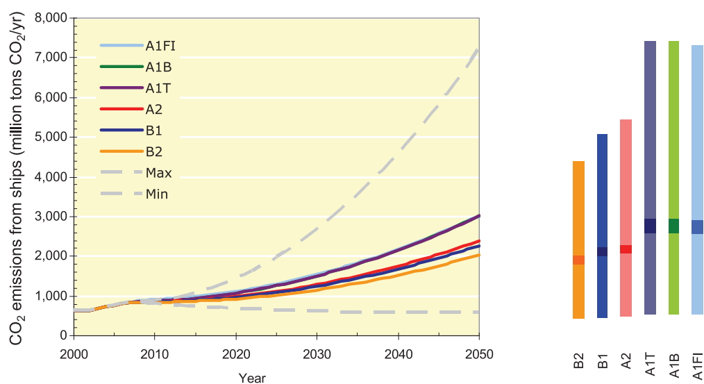
Figure 7.8 Trajectories of the emissions from international shipping. Columns on the right-hand side indicate the range of results for the scenarios within individual scenario families
