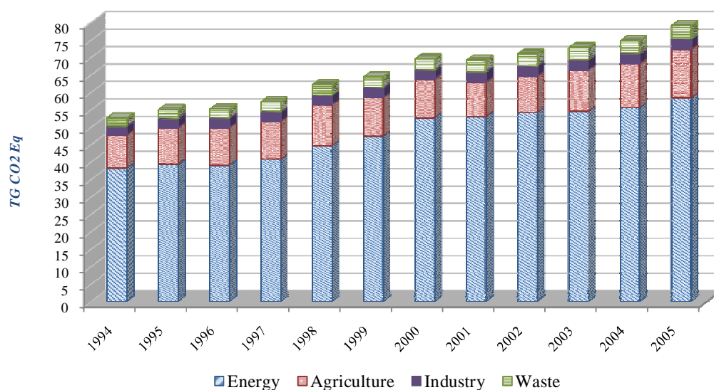
Fig. 2.4 GHG Emissions according to Sector from 1994 to 2005
