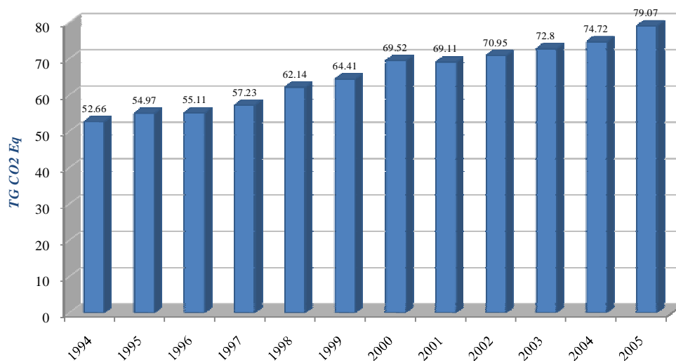
Fig. 2.1 Total Emissions of GHG from 1994 to 2005
