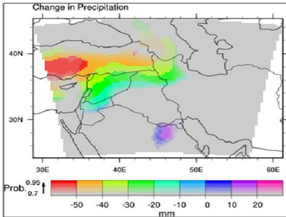
Fig. 3.17 Probability of Changes in Precipitations by Amount (hue) and Significance (sat).
