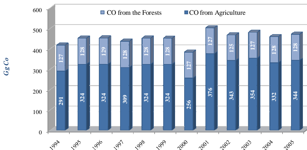
Fig. 2.22 Emissions of CO by LUCF
