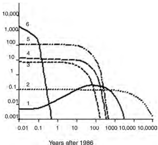
Figure 15.1. Total additional radioactivity (in petabecquerels) in the global environment after the Chernobyl catastrophe: (1) Am-241, (2) Pu (239 + 240), (3) Pu-241, (4) Sr-90, (5) Cs-137, (6) I-131 (Mulev, 2008).
