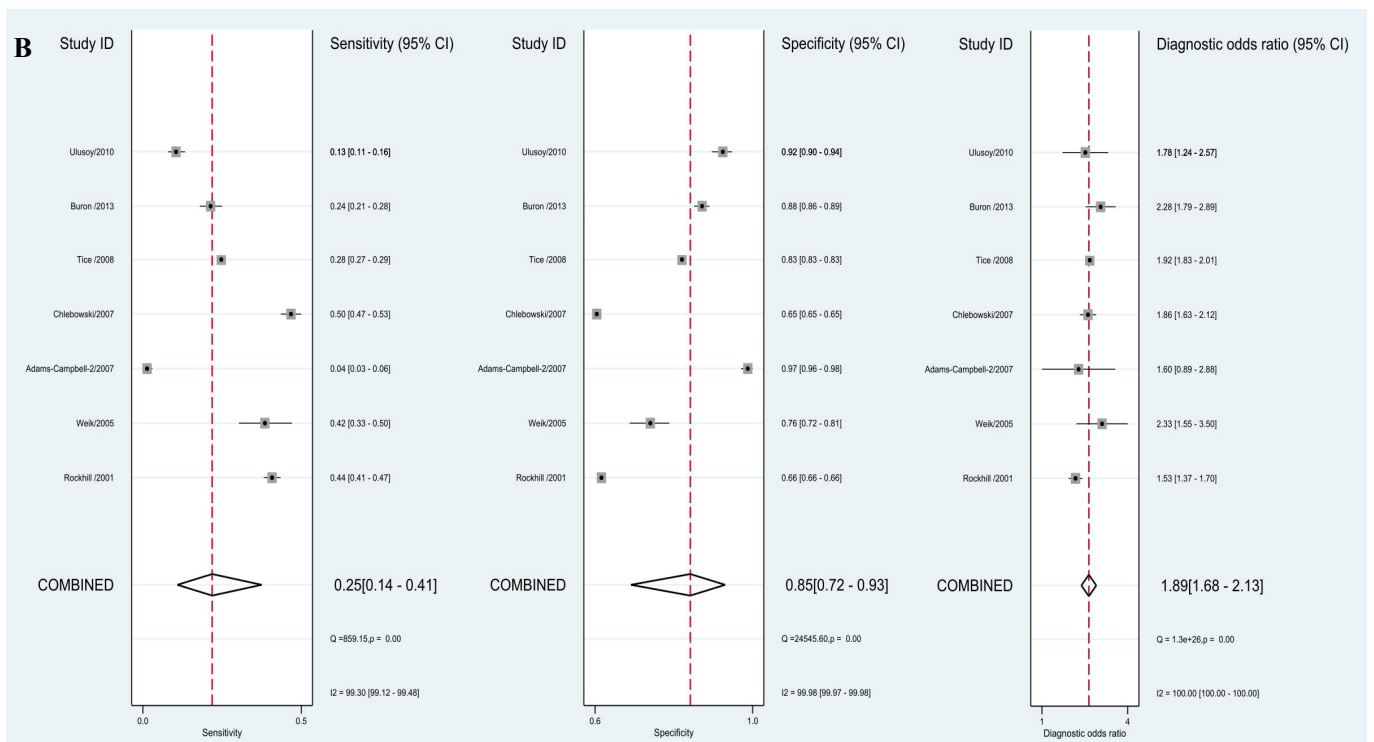
Additional file 19. The pooled sensitivity, specificity and diagnostic odds ratio of the Gail model 1 (A) and the Caucasian-American Gail model 2 (B) after excluding the studies published in Chinese.
