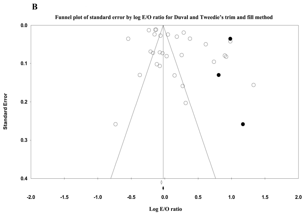
Additional file 2. Funnel plot of the calibration of the Gail model (A) and the funnel plot adjusted by trim-and-fill method (B).
