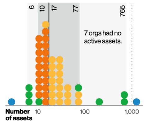
Figure 30. Number of internet-facing assets in randomly selected organizations (n=85) Each dot represents 2% of organizations
