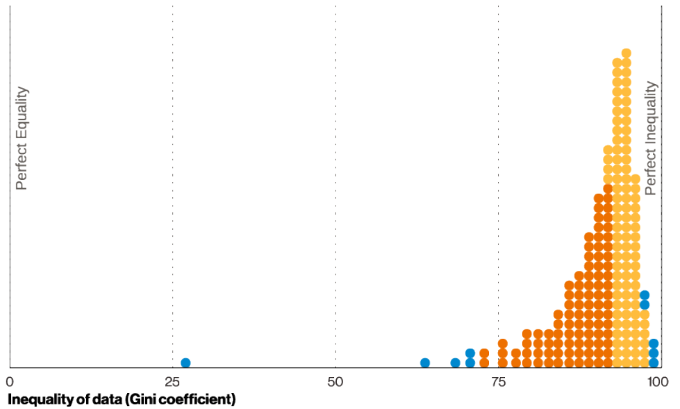
Figure 77. Inequality of Malware phishes per day (n=1,767) Each dot represents 0.5% of organizations
