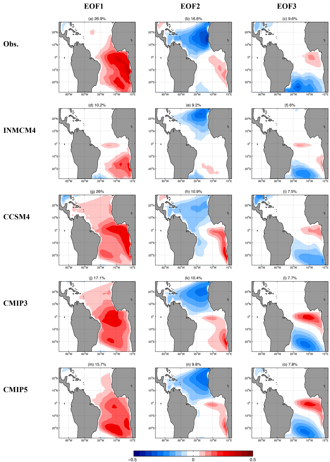
Supplemental Fig. 3 First three leading EOF patterns, as in Fig. 10, but of high-pass SSTA in the Tropical Atlantic for a selection of model simulations and observations. In addition to the observations, the CMIP3 and CMIP5 super models, the models with the largest (INMCM4) and smallest (CCSM4) RMSE EOF value are shown.
