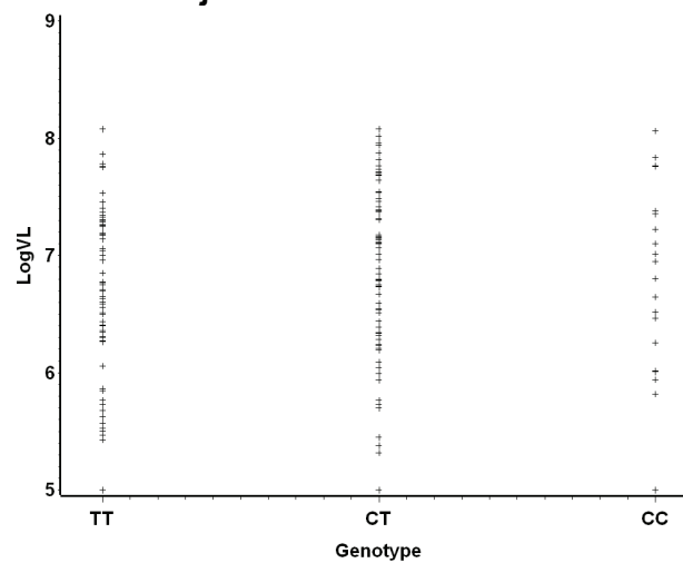
Figure S1. The effect of rs12979860 genotype on HCV viral load. A) All patients, B) white subjects, C) Black subjects. The results indicate that there is no correlation between HCV viral load and rs12979860 genotype ( R^2 = 0.0015, 0.0006, 0.0055 for all subjects, whites and blacks respectively).
