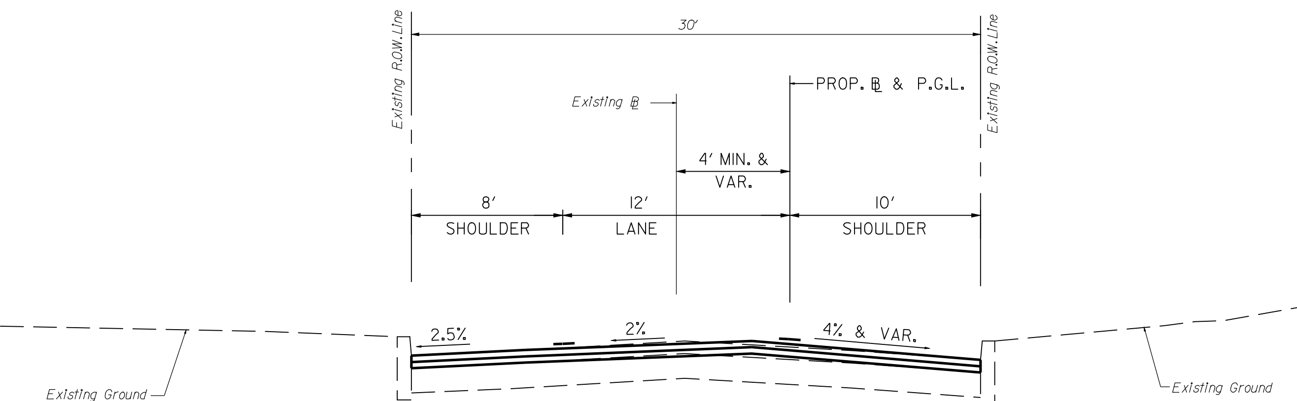
ROUTE 23 NB NORMAL SECTION STA. 62+50 TO 80+00
