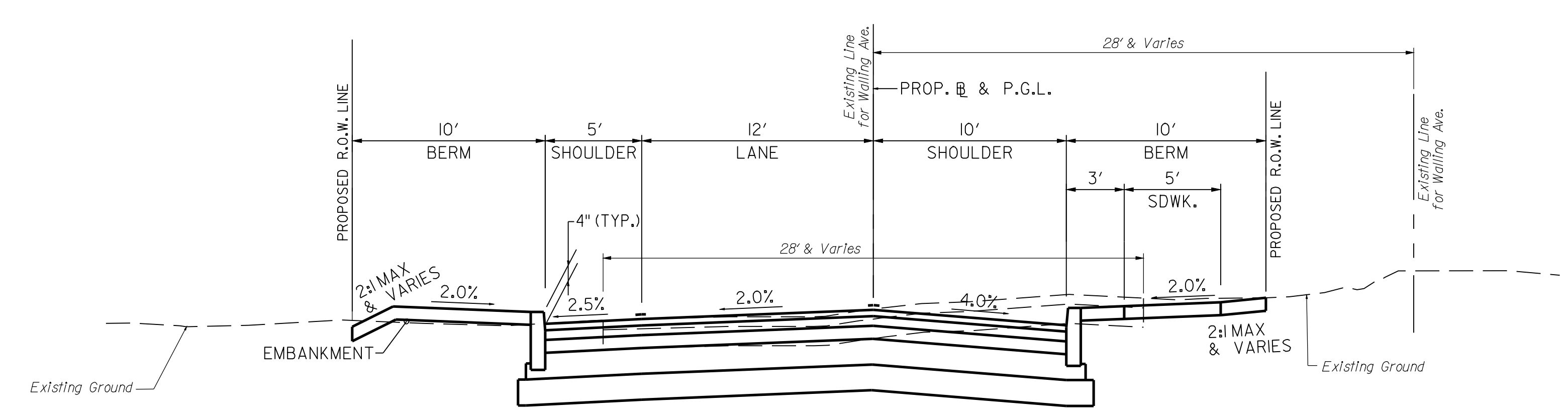
ROUTE 23 SB NORMAL SECTION STA. 42+00 TO 46+33
