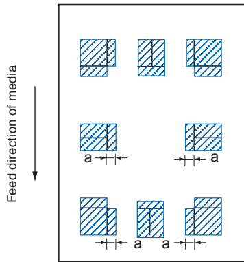
MARK TYPE 1 (There are central registration marks.)
