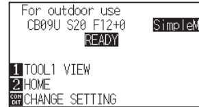
Display of Default Screen (Simple mode)
