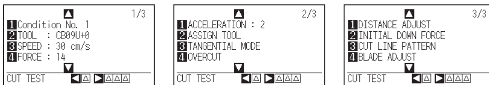
CONDITION screen (1-3) : (Normal mode)
