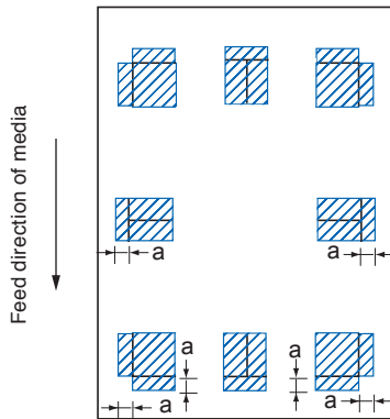
MARK TYPE 2 (There are central registration marks.)
