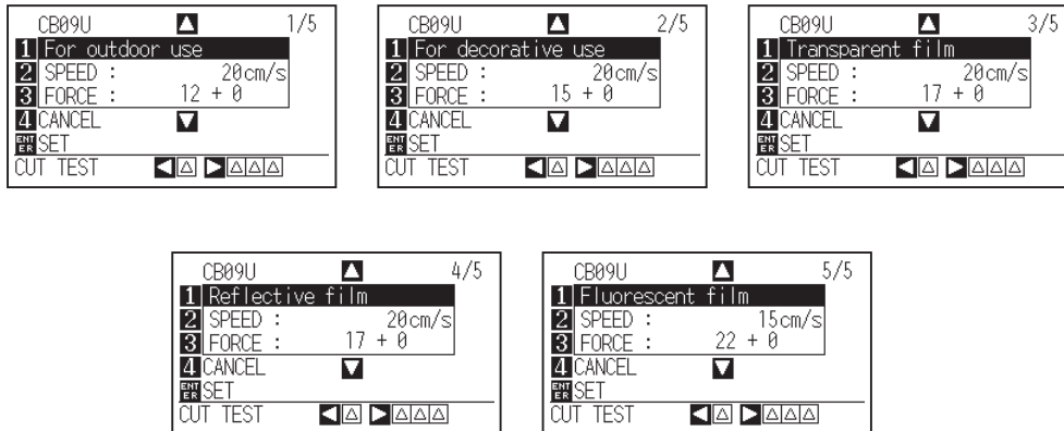
CONDITION screen (1-5): (Simple mode)
