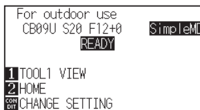
READY screen (Simple mode)
