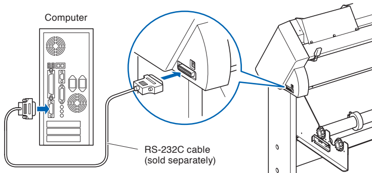
Connection via RS-232C interface
