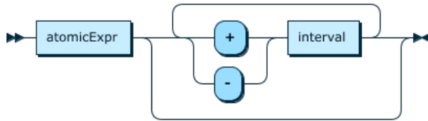
Figure 12.22 intervalExpr
