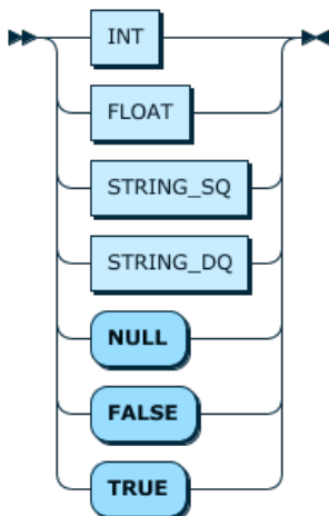
Figure 11.35 Literal
