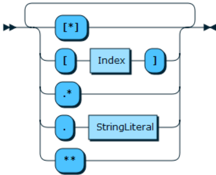
Figure 11.34 DocPath
