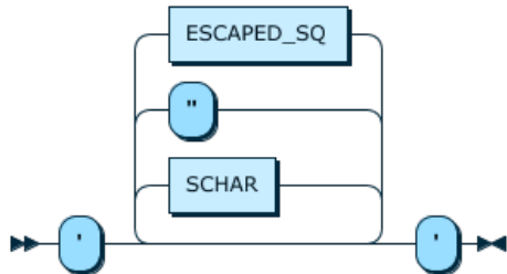
Figure 12.40 STRING_SQ
