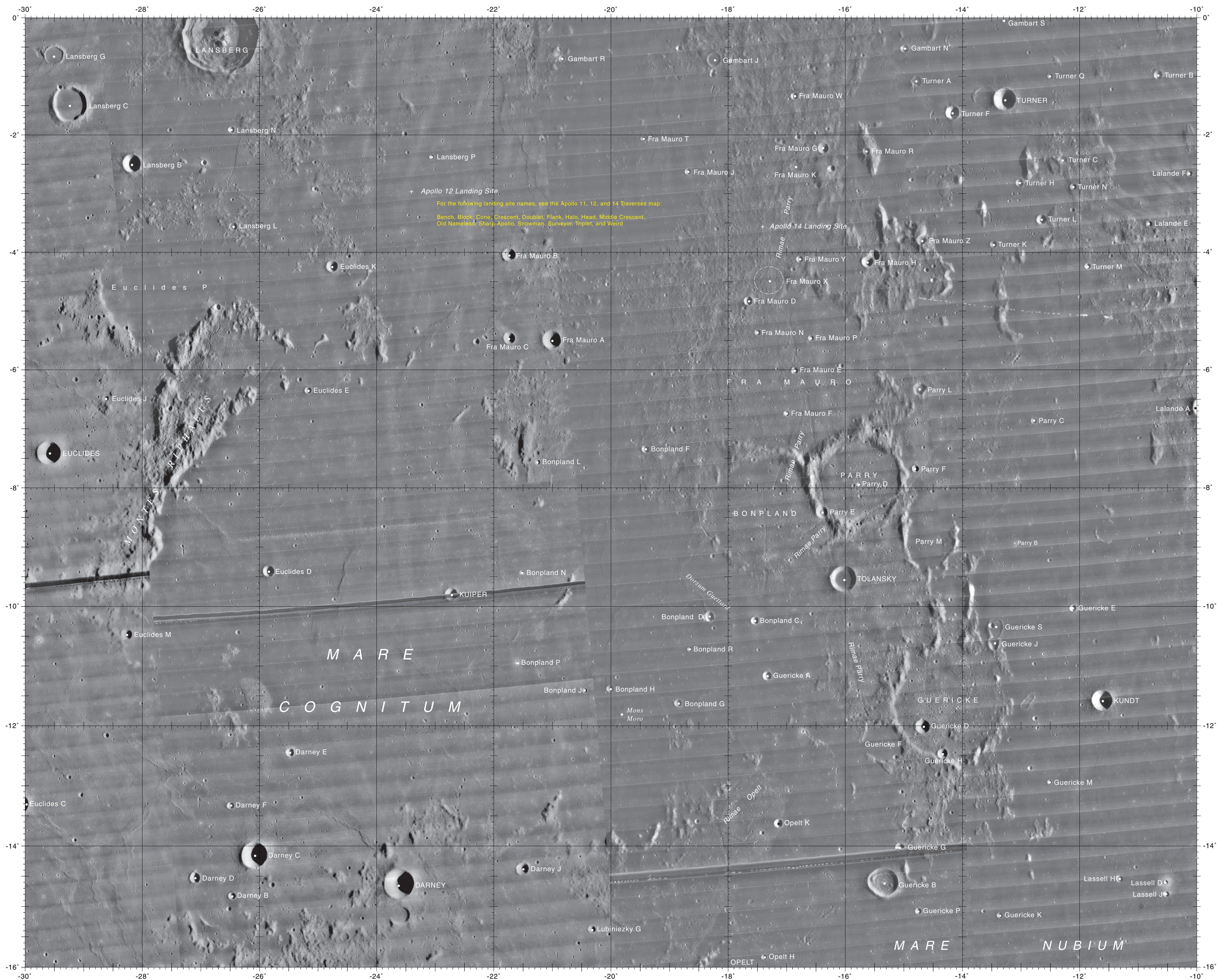
LAC 76 Scale 1:1,000,000 Mercator Projection
