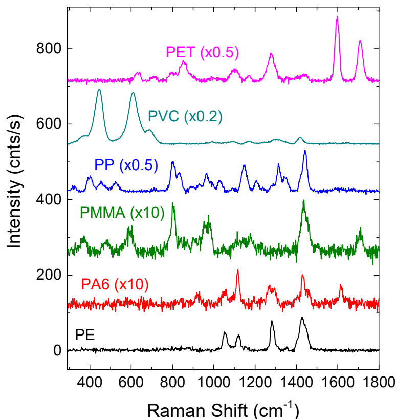
Figure 8: Raman spectra of optically trapped micro- and nano- plastics made of different materials in seawater. Particle dimensions are: PET 2.6 \mu\text{m} , PVC 3 \mu\text{m} , PP 2.8 \mu\text{m} , PMMA sub-micron, PA6: Submicron, PE 2 \mu\text{m} . Laser wavelength 633nm. Power 15 mW, before objective. Integration times are 20 s (2 acquisitions) for PE and PVC, 60s (2 acquisitions) for PA6 and PMMA, 4s (2 acquisitions) for PP, and 2s (2 acquisitions) for PET. Spectra are background-subtracted, rescaled (factors indicated in parentheses) and offset in order to make intensities compared.
