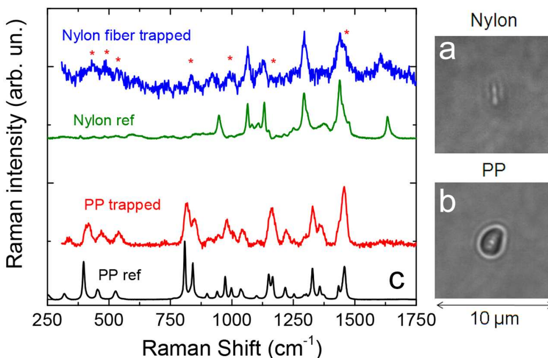
Figure 12. Optical images of a nylon fiber (a) and a spheroidal PP particle (b) dispersed in seawater. (c) Raman spectra of the optically trapped particles (blue and red) compared with the reference spectra (green and black lines) acquired on bulk samples. The red asterisks highlight additional peaks in the nylon spectrum that can be attributed to PP. Excitation wavelength 633nm, power 15 mW before objective, integration times 4s, 2 acquisitions.
