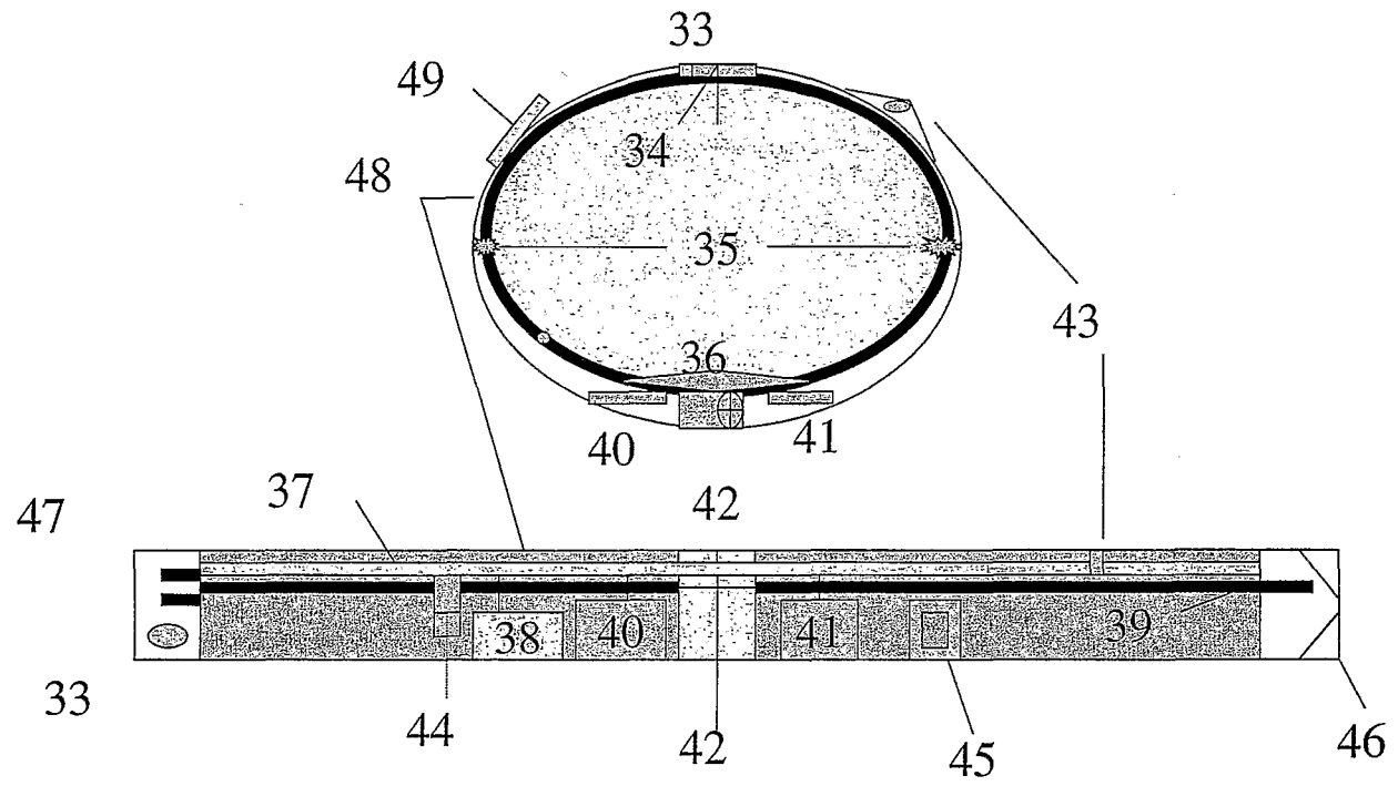
FIG. 33 BELT, CLASP, COLLAR OR BRACELET SECURITY SYSTEM
