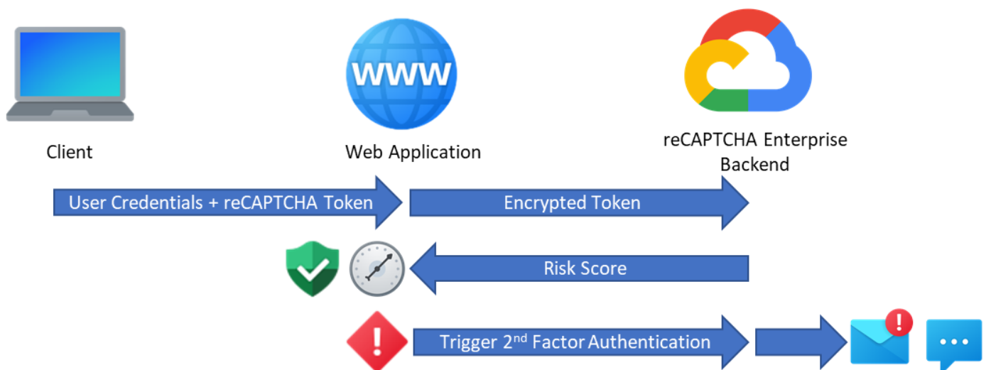
Figure 9. Using reCAPTCHA Enterprise to Protect from Account Takeovers
