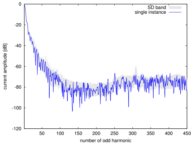
(a) The noisy spectrum of a single instance.
