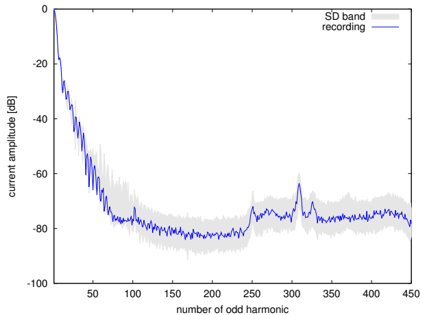
(b) The mean spectrum of multiple instances.
