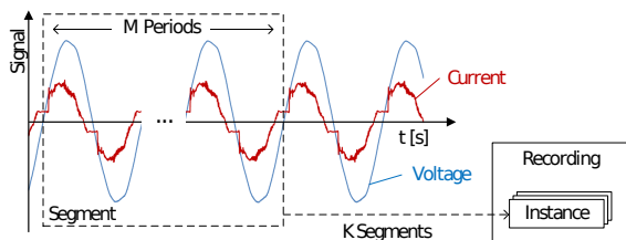
Figure 3: The segmentation process of the PISI .
