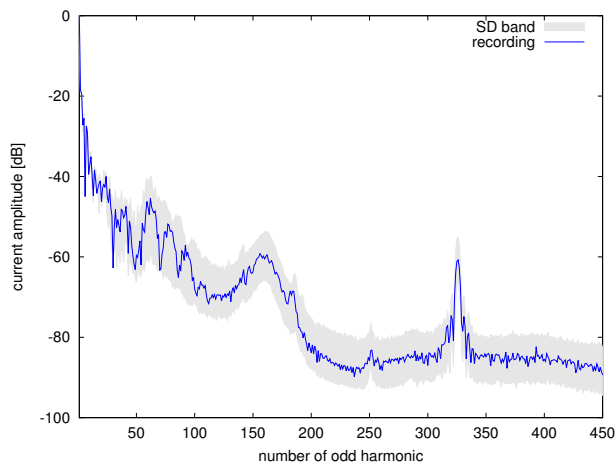
Figure 5: The variance of the spectrum of a monitor over a period of one week.
