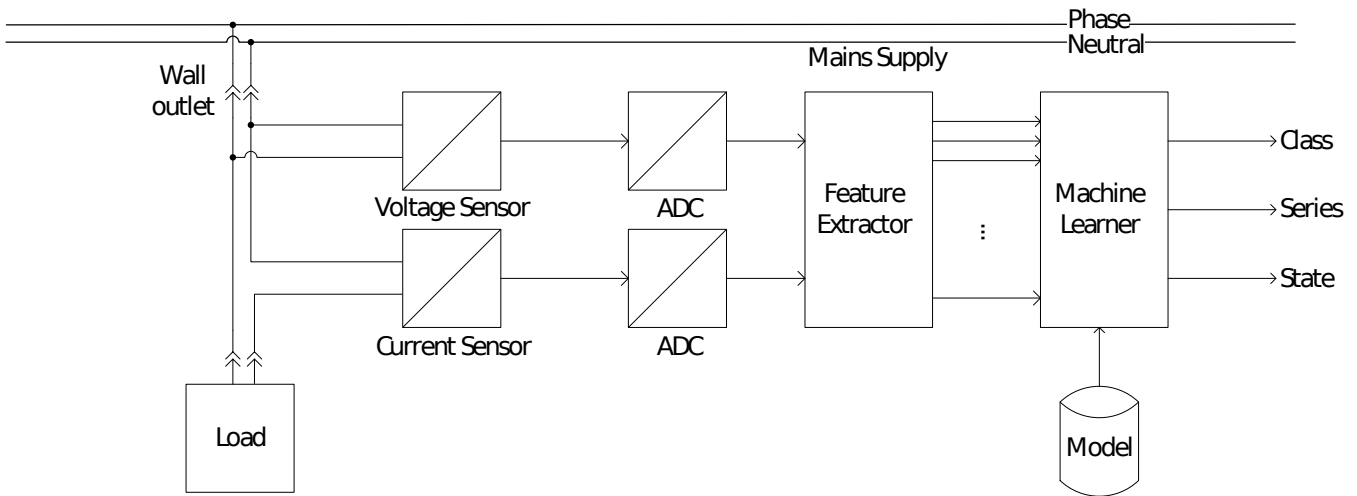
Figure 1: A schematic system overview: Our hardware board measures the voltage and the current of the load. The resulting signals are then converted to the digital domain and post processed by a machine learning toolkit.
