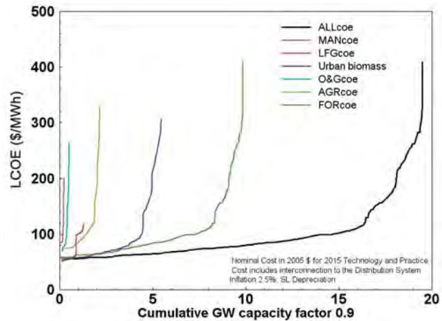
Figure 20. Capacity supply curves for biomass based on 18 western states. Key to figure curves: Man = Manure, LFG = Landfill Gas, Urban Biomass = Municipal Solid Waste, O&G = Orchard and Grapes (California only), AGR = Agricultural Residues, FOR = Forestry Resources.
