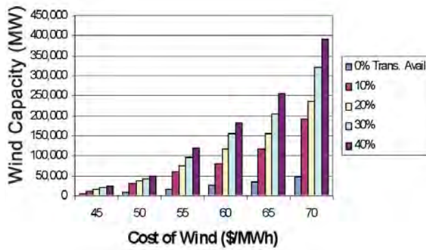
Figure 5. Impact of transmission availability on wind supply.
