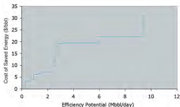
Figure 3. Petroleum efficiency cost curve (2025).
