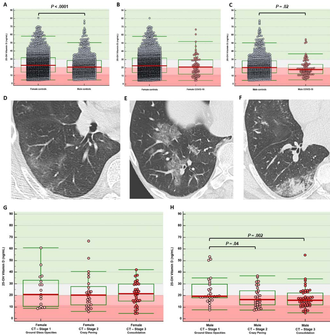
395 Figure 2: 25(OH)D levels in male and female COVID-19 patients and age/season-matched controls 396 and stratification by COVID-19 disease stage Panels A-C: Box-and-Whisker plots showing median 397 (red line) serum 25(OH) levels and interquartile ranges (green box) in (A) season- and age-matched 398 female (n=1718) versus male (n=999) diseased controls; (B) female COVID-19 patients on admission 399 (n=77) versus female controls; (C) male COVID-19 patients on admission (n=109) versus male 400 controls. Panels D-F: representative images of radiological stages of COVID-19 lung disease with 401 predominantly (D) ground-glass opacities in early stage; (E) crazy paving patterns in progressive stage 402 2; and (F) consolidation in peak stage 3. Panel G-H: box-and-whisker plots of 25(OH)D in (G) 403 female COVID-19 patients and (H) male COVID-19 patients grouped according to radiological stage. 404 Background color in box plots indicates normal vitamin D status (green, 25(OH)D > 30 ng/mL), 405 vitamin D deficiency (pale red, 25(OH)D < 20 ng/mL), severe vitamin D deficiency (darker red, 406 25(OH)D < 12 ng/mL) and a gray zone (20 ng/mL ≤ 25(OH)D ≤ 30 ng/mL). P values indicate statistical
