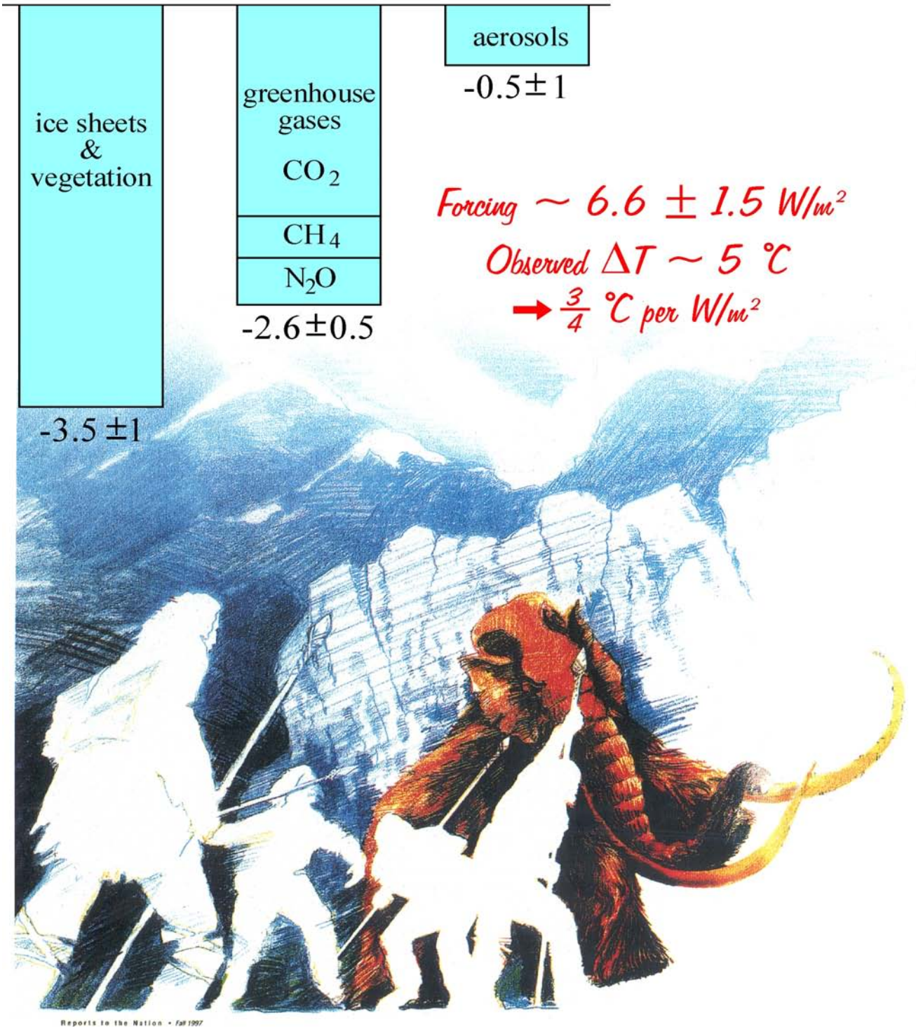
Figure 3. Climate was dramatically different than today during the last ice age, which peaked 20,000 years ago. Global climate forcing was about 6½ W/m 2 less than in the current inter-glacial period. This forcing maintained a planet 5°C colder than today. [Drawing from Reports to the Nation , Fall, 1997.]
