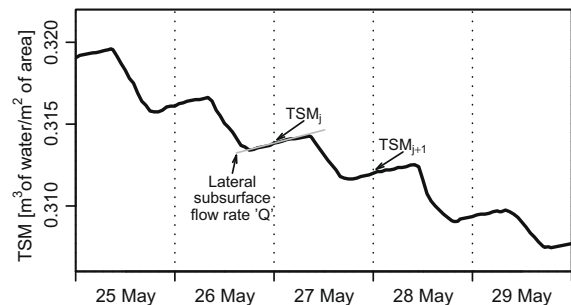
Fig. 13. Total soil moisture (TSM) versus time in the groundwater discharge area. The subsurface flux is the positive slope of the line between midnight and 4 a.m. (after Nachabe et al., 2005).
