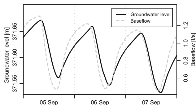
Fig. 3. ET-induced diel signal in groundwater level and streamflow rate, Hidegvíz Valley experimental catchment near Sopron, Hungary, 2005.
