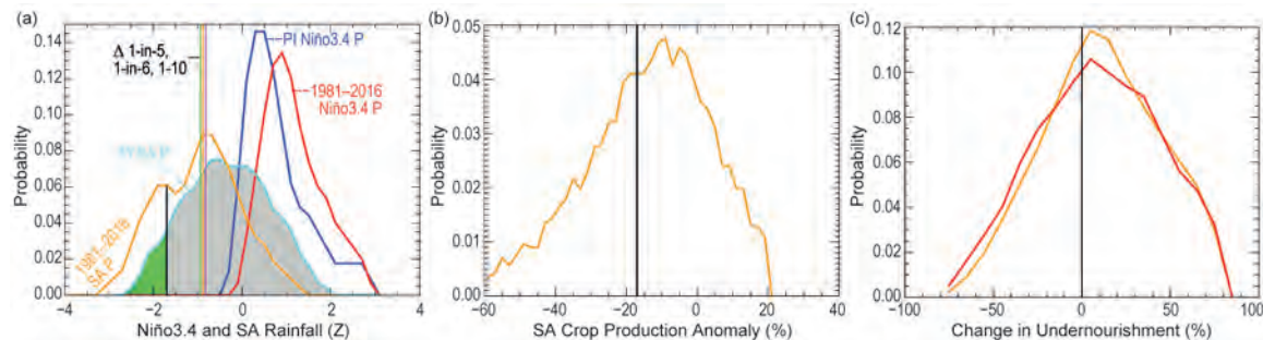
FIG. 18.2. (a) Precipitation attribution results. Standardized CESM SA and Niño-3.4 MSENEnsemble precipitation (Z) PDFs for PI and 1981–2016 Historic ensembles. Historic MSENEnsemble was based on 15% of 40 simulations for 36 years (216 El Niño events). Also shown are results based on 10% and 20%. PI ensemble used 15% of 1680 years (252 El Niño events). Green and gray shading indicates the probability of the observed -1.7Z drought occurring within the PI distribution. (b) Bootstrapped distribution of SA crop production anomalies (%), based on the PI and Historic SA precipitation distributions from (a), and the slope coefficient sampling distribution. Anomalies based on 2008–13 averages. (c) PDFs of changes in undernourishment (%) in Zimbabwe and Malawi, based on (b) and an FAO percent undernourished estimation procedure.
