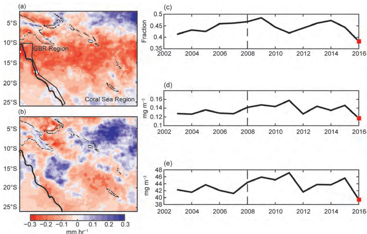
FIG. 28.2. Satellite-derived observational products for JFM precipitation anomalies in the Coral Sea region for (a) 2016 and (b) 1998 ( \text{mm hr}^{-1} ; relative to 1998–2016 climatology from TRMM rainfall retrievals for 1998–2016), (c) cloud area fraction (%; daytime) from AIRS/Aqua retrieval, 1^{\circ} \times 1^{\circ} for 2002–16), (d) chlorophyll-a concentration ( \text{mg m}^{-3} ; from MODIS–Aqua 4-km monthly data), and (e) particulate organic carbon ( \text{mg m}^{-3} ; from MODIS–Aqua 4-km monthly data). The general location of the GBR is shown in (a).
