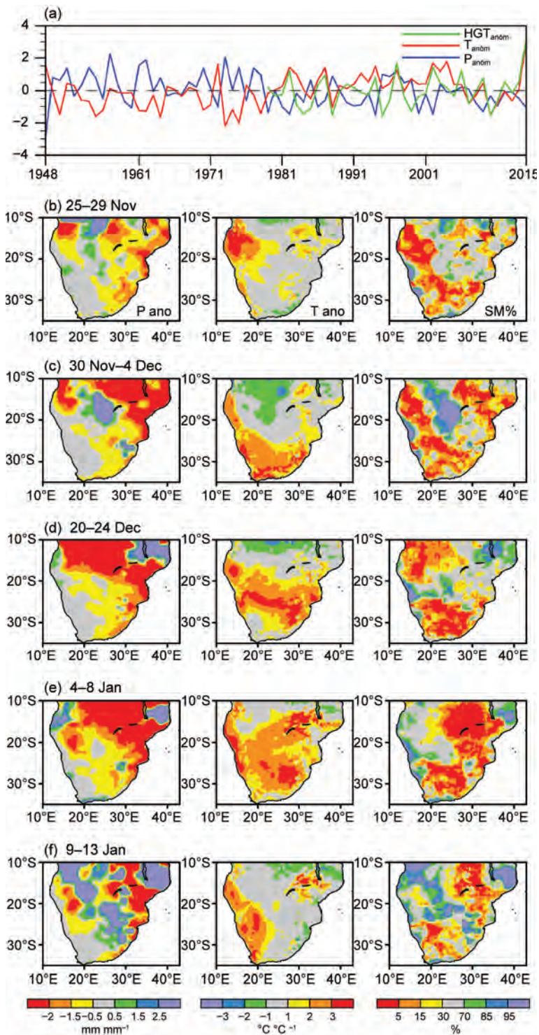
FIG. 17.1. (a) Interannual variations of standardized Dec–Jan mean precipitation (blue), temperature (red) and 500-hPa geopotential height (green) anomalies averaged over southern Africa ( 10^{\circ} – 40^{\circ} E, 10^{\circ} – 35^{\circ} S) during 1948–2016. (b)–(f) Flash drought snapshots of standardized pentad-mean precipitation (left; \text{mm mm}^{-1} ) and surface air temperature (middle; ^{\circ}\text{C } ^{\circ}\text{C}^{-1} ) anomalies and soil moisture percentiles (right; %) during Dec–Jan 2015/16. Precipitation and temperature anomalies were divided by std. dev. of the 1961–2012 climatology.
