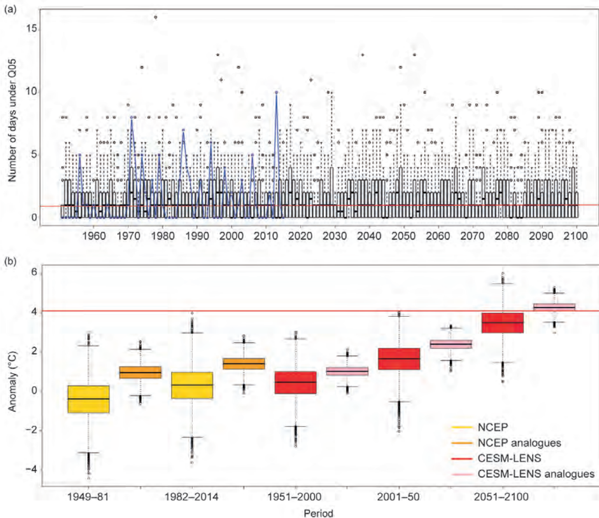
FIG. 15.2. (a) Number of days per year with SLP distances below 5th percentile of distribution of daily distances to closest December 2015 day. Box plots show dispersion of CEM ensemble members. Blue lines-dots are values for NCEP reanalysis. Red line is (nonsignificant) linear trend of median of CEM ensemble members. (b) Box plots of control distributions (respectively uchronic distributions) of anomalies of national temperature index relative to observed climatology of this index between 1948 and 2015, in yellow (orange) using NCEP and in red (pink) using CEM-LENS subsets.
