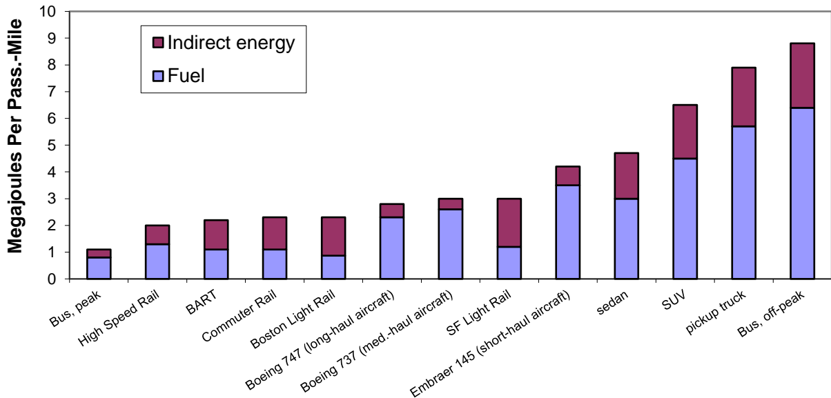
Figure 20 Lifecycle Energy Consumption (Chester and Horvath 2008)
