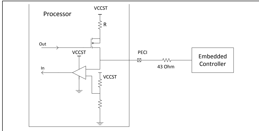
Figure 2-10. Example for PECEC Connection
