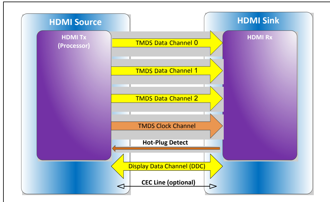
Figure 2-8. HDMI* Overview
