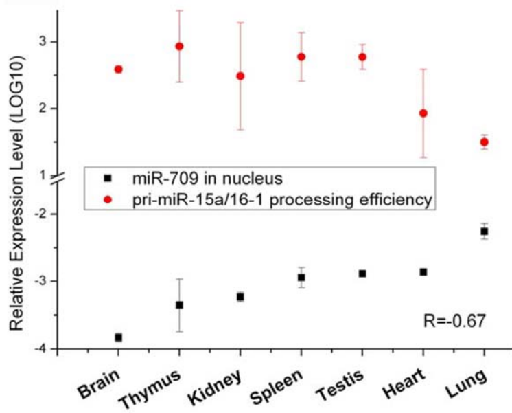
Supplementary information, Figure S5 The correlation between nuclear miR-709 and pri-miR-15a/16-1 processing efficiency in mice (seven tissues including testis, brain, spleen, thymus, kidney, heart, and lung). R, Pearson correlation coefficient.
