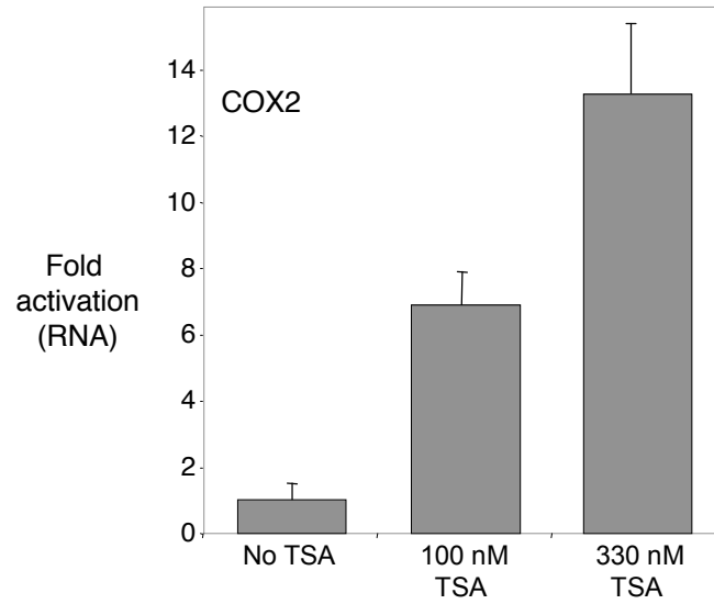
Supplementary Fig. 3. Treatment of MCF-7 cells with TSA yields increases COX-2 expression. QPCR showing activation of cyclooxygenase-2 (COX-2) by the histone deacetylase inhibitor (HDAC) trichostatin-A (TSA). Fold activation is relative to controls cells that were not treated with TSA.
