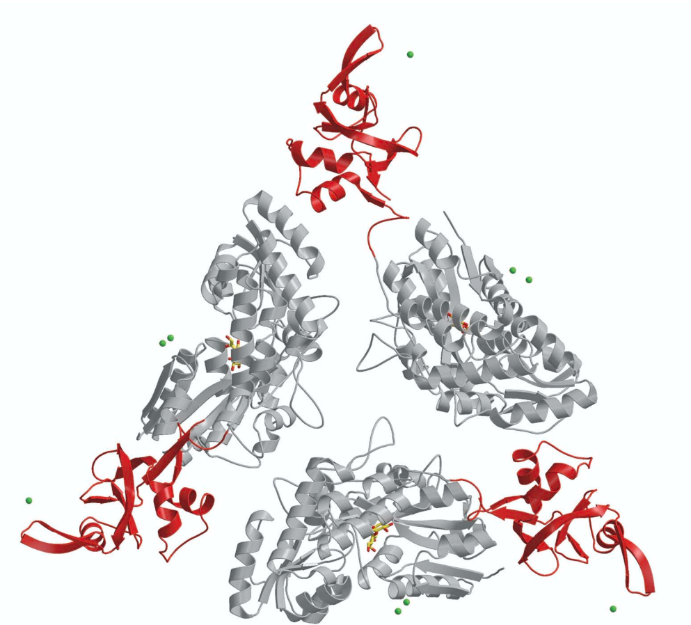
Supplementary Figure 1 Ribbon diagram of the MBP-PAZ fusion protein crystal structure. Shown are the three molecules in the asymmetric unit, with MBP in gray, Ago2-PAZ in red, the maltose in stick representation and Ni 2+ ions as green spheres. The orientation of the PAZ domain with respect to MBP is different in each molecule.
