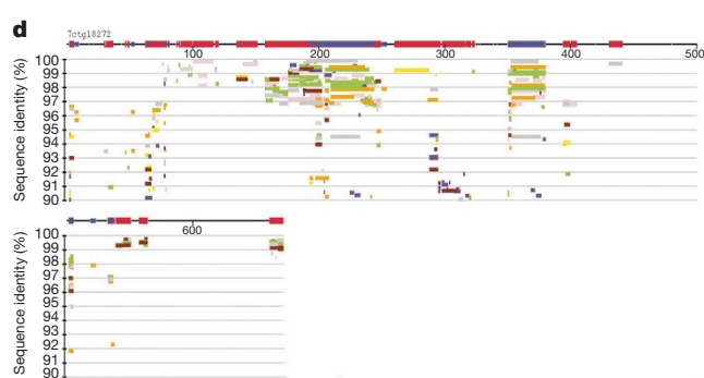
sequence duplication is indicated (with a distinct colour) relative to per cent nucleotide identity for the duplicated segment (y axis). Black bars show the relative locations of large blocks of heterochromatic sequences (alpha, gamma and HSAT sequence). a , An active pericentromeric region on chromosome 21. b , An ancestral region from Xq28 that has contributed various 'genetic' segments to pericentromeric regions. c , A pericentromeric
