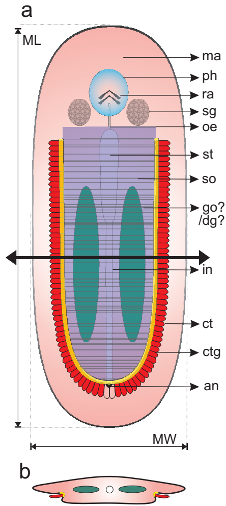
Supplementary Figure I. Schematic model of Odontogriphus omalus . a , dorso-ventral view. b , cross section at mid-body level. an=anus, ct=ctenidia, ctg=ctenidia groove, dg?=digestive glands?, go?=gonads?, in=intestine, ma=mantle ML=maximum length, MW= maximum width, oe=esophagus, ph=pharynx and mouth area, ra=radula, sg=salivary glands, so=sole, st=stomach.
