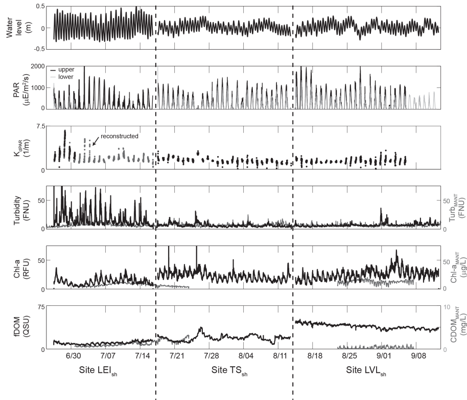
Figure 2. Time series of water level, photosynthetically active radiation (PAR), light attenuation over the PAR spectrum ( K_{dPAR} ), turbidity, chlorophyll a fluorescence (chl a ), and fluorescing dissolved organic matter (fDOM) for each site, starting from the south on the left. The grey trace in bottom three panels are reference values from site Mantoloking.
