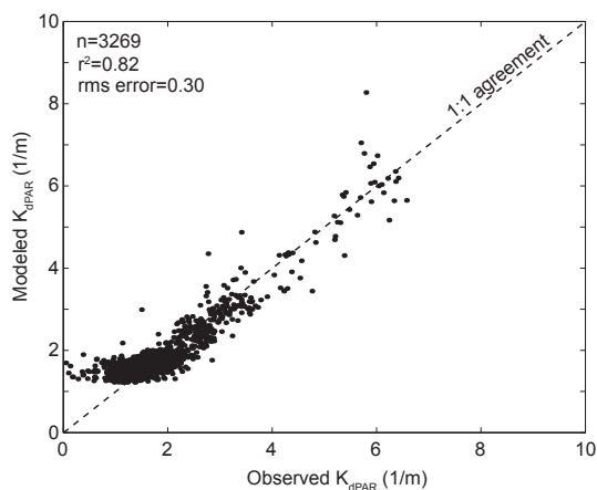
Figure 8. Agreement between observed K_{dPAR} over the PAR spectrum and the spectral attenuation model of Gallegos et al. (2011).
