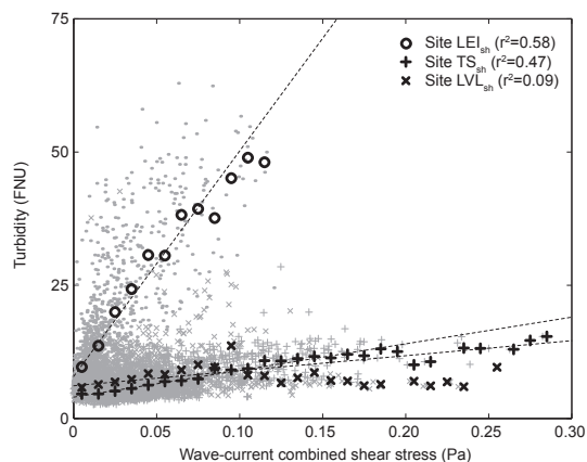
Figure 9. Relationship between wave–current combined shear stress and turbidity at three shoal sites; darker symbols are instantaneous data binned and averaged in 0.01 Pa intervals. Site LEI sh demonstrates enhanced resuspension as compared to other sites under similar stress conditions; surficial sediment distribution indicates a higher abundance of fine material in the southern part of the system.
