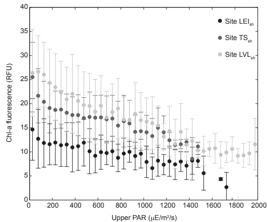
Figure 5. Relationship between binned near-surface irradiance in the PAR spectrum (400–700 nm) and measured chlorophyll a fluorescence. Bounds are one standard deviation of measured fluorescence within each bin. Fluorescence decreases with irradiance at all shoal sites, indicating substantial non-photochemical quenching (NPQ) of fluorescence.
