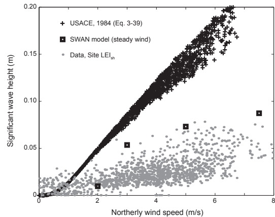
Figure 11. Measured and modeled wave-height response to wind at site LEI sh ; the USACE formulation neglects spatial variation in bathymetry and the SWAN model does not include the influence of tidal currents and assumes a constant, uniform wind field.
