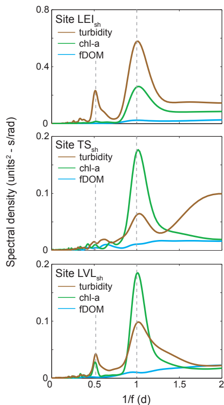
Figure 4. Spectral density of turbidity, chlorophyll a , and fDOM time series from three shoal sites. Dashed lines correspond to M_2 tidal period (0.5175 d) and the diurnal period (1 d). Note the difference in y axis scaling at LEI_{sh} in comparison to the other two sites.
