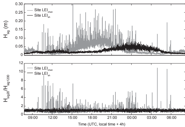
Figure 10. Example of a single day of significant wave height ( H_{sig} ) data from sites LEI chan and LEI sh , and the ratio of 20 s window significant wave height ( H_{sig20} ) to 1200 s window significant wave height ( H_{sig1200} ). The latter metric is used to identify vessel wakes, which are observed frequently at site LEI chan , but seldom at site LEI sh .
