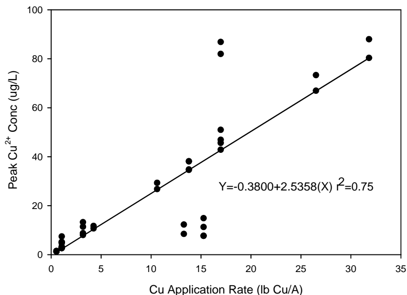
Figure 3 - Correlation of Peak Cu 2+ Concentrations in the Standard Small Water Body with Application Rates
