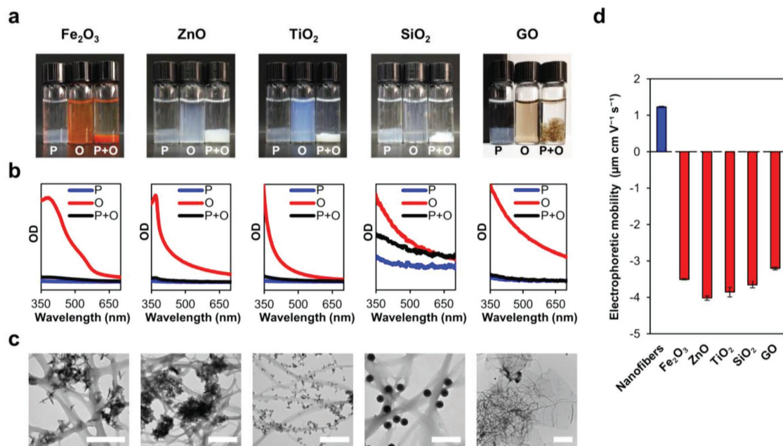
Figure 1. Binding of oxide particles to peptide nanofibers. a) Photographs of nanofiber dispersions, different dispersions of oxide particles, and peptide nanofiber-oxide mixtures. P and O denote peptide nanofibers and oxide particles, respectively. Photographs were taken following 3 h incubation. A sedimenting floccule is seen at the bottom of the vial in nanofiber dispersions and nanofiber-oxide mixtures, but not in oxide dispersions. b) UV-vis spectra of liquid bulk samples corresponding to panel (a). c) TEM images of floccule samples from the nanofibers-oxide mixtures corresponding to (a). Scale bars are 500 nm except for GO, where scale bar is 2 \mu\text{m} . d) Electrophoretic mobility of peptide nanofibers and oxide particles. Under the experimental conditions, attraction between opposite electrostatic charges drives the binding of oxide particles to the sedimenting peptide nanofibers. Data represent mean \pm standard error of the mean ( n = 3 samples).
