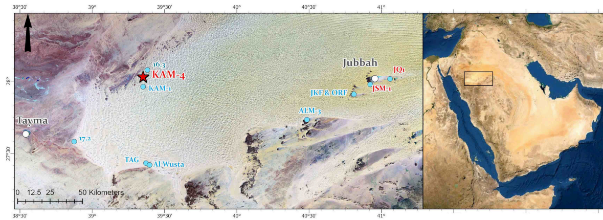
Supplementary figure 1. Location of KAM-4 and Jubba sites (JSM-1 and JQ-1) in the Nefud Desert in northern Saudi Arabia. Other regional sites discussed in the text are also shown.
