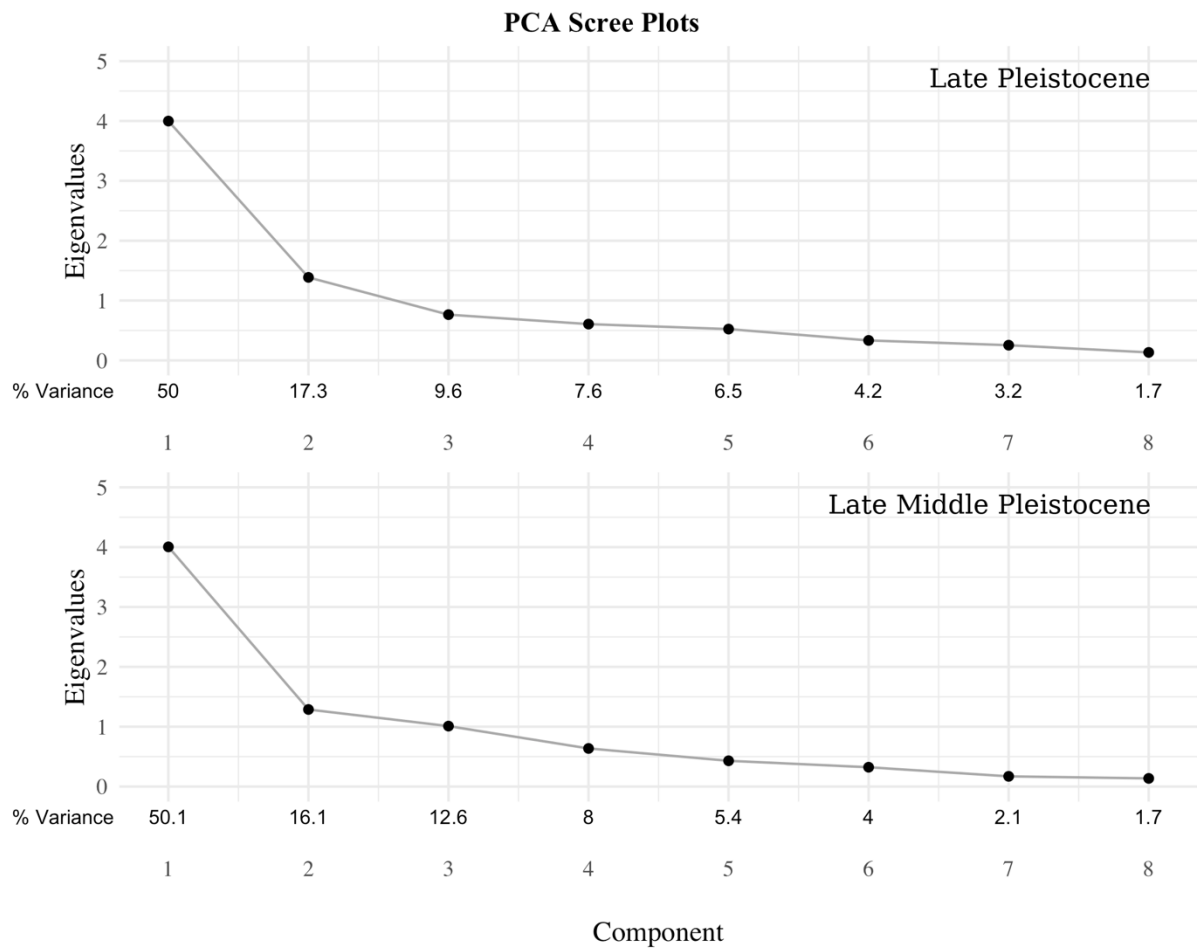
Supplementary figure 37. Scree plots for the two PCA analyses.
