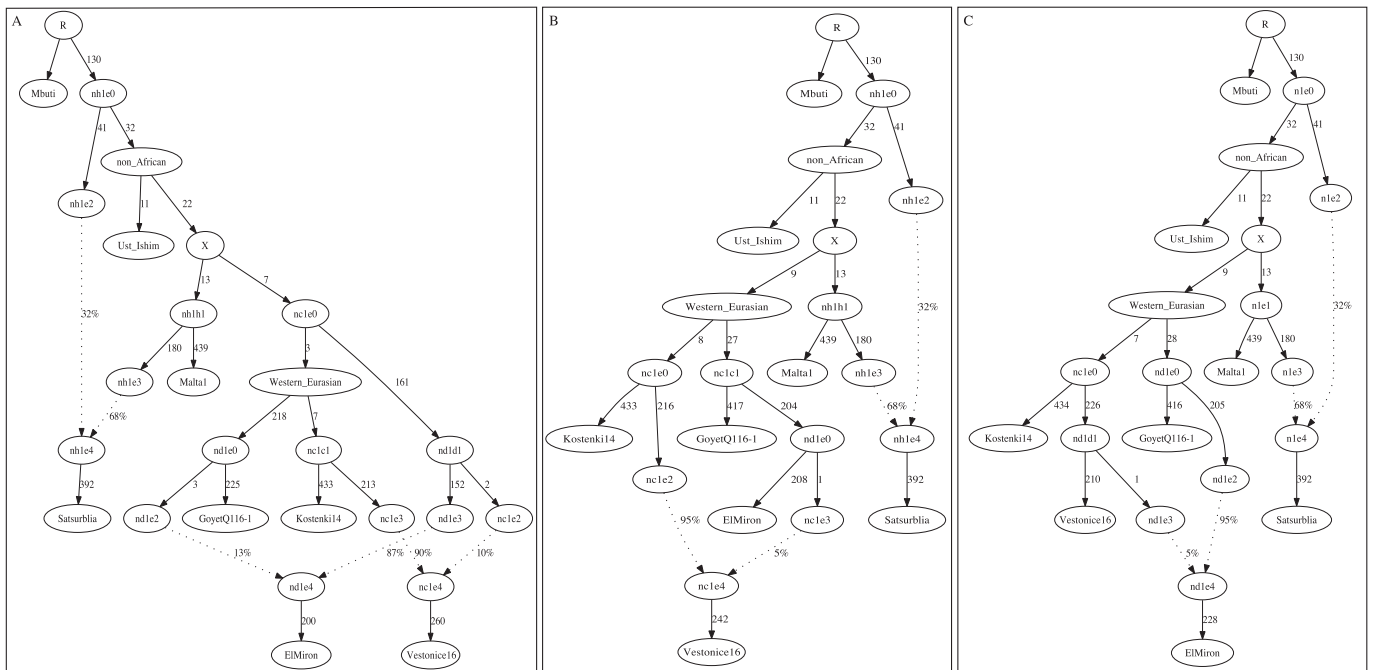
Extended Data Figure 4 | Three admixture graph models that fit the data for Satsurblia, an Upper Palaeolithic individual from the Caucasus. These models use 127,057 SNPs covered in all populations. Estimated genetic drifts are given along the solid lines in units of f_2 -distance (parts per thousand), and estimated mixture proportions are given along the dotted lines. All three models provide a fit to the
