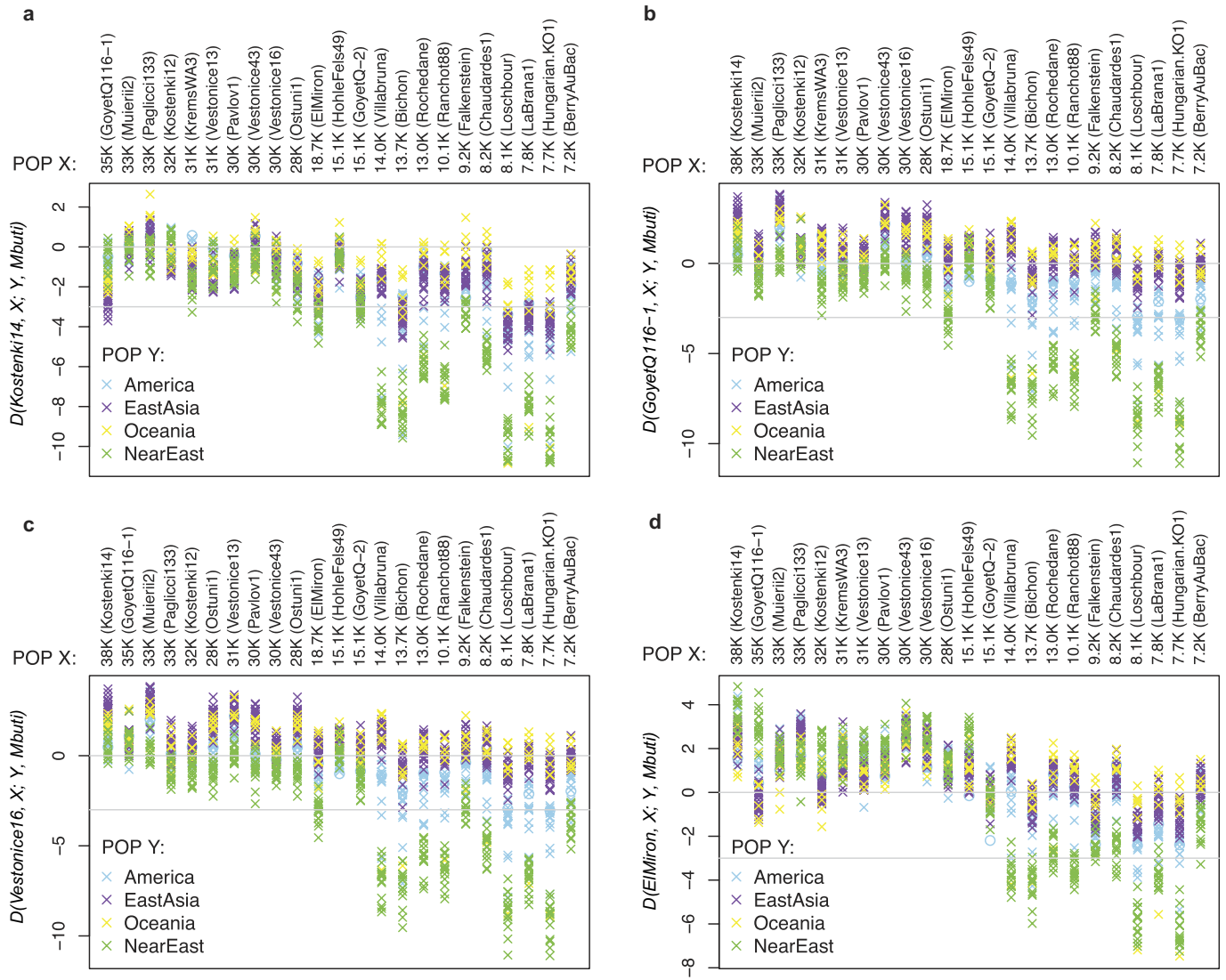
Extended Data Figure 3 | Studying how the relatedness of non-European populations to pairs of European hunter-gatherers changes over time. Statistics were examined of the form D(W, X; Y, Mbuti) , with the Z-score given on the y axis, where W is an early European hunter-gatherer, X is another European hunter-gatherer (in chronological order on the x axis), and Y is a non-European population (see legend).
