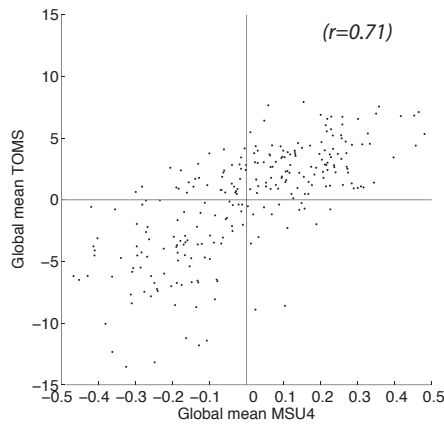
c) Global mean T4 and TOMS/SBUV ozone
