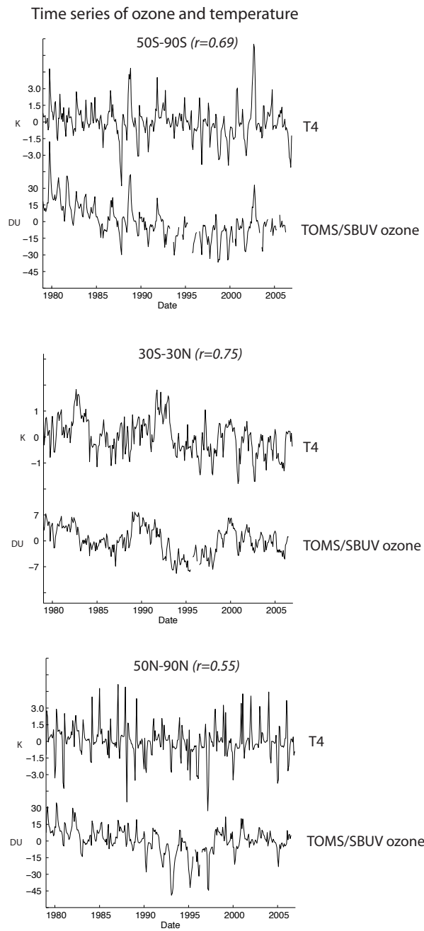
Figure 6. Time series of zonal-mean, monthly-mean TOMS/SBUV column ozone and T4 anomalies for latitude bands indicated. Values of zero denote the long-term mean.
