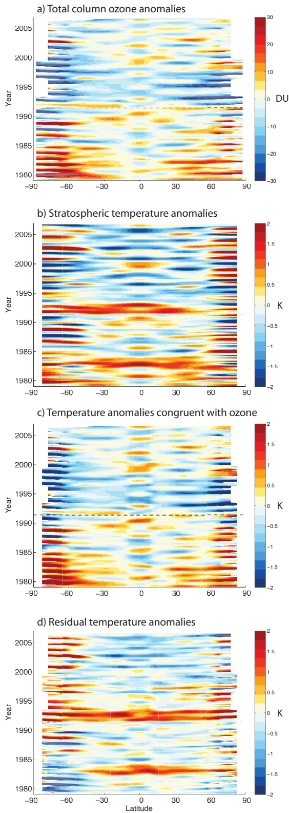
Figure 3. Panels a) and b): Zonal-mean, monthly-mean time series of (a) TOMS/SBUV column ozone anomalies and (b) T4 anomalies. The horizontal dashed line denotes the Mt. Pinatubo eruption date. Contour plots are smoothed with a 5 month running mean filter for display purposes only. Note the data are in anomaly form and hence do not exhibit a seasonal cycle. Panels c) and d): As in panels a) and b) but for (c) the components of the zonal-mean, monthly-mean T4 anomaly time series that are linearly congruent with the TOMS/SBUV column ozone anomaly time series; and (d) the associated ozone-residual T4 anomaly data. Note the fitted and residual time series are found as a function of latitude band and are given by Eq. 2.
