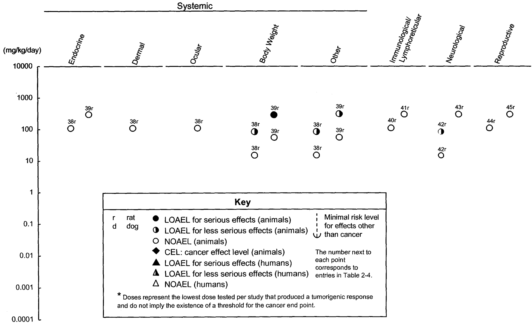
Figure 2-2. Levels of Significant Exposure to Formaldehyde - Oral (cont.) Chronic ( \geq 365 days)
