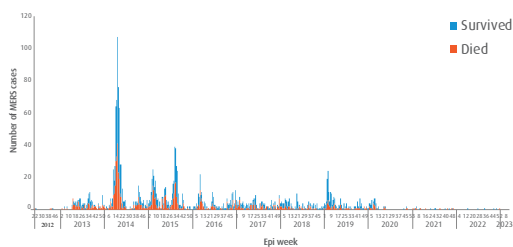
Fig. 3. MERS cases per week of onset in Saudi Arabia, June 2012 – March 2023
