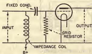
FIG. 43. — Impedance-coupled radio-frequency circuit.
