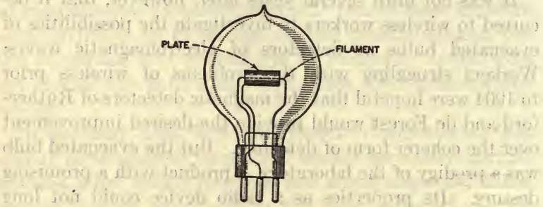
FIG. 13.—The Fleming valve, or two-electrode tube. The filament conductor passes through a tubular plate element.
