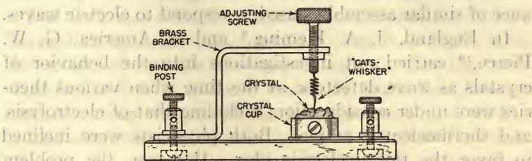
FIG. 11.—Crystal detector employing silicon or galena.
