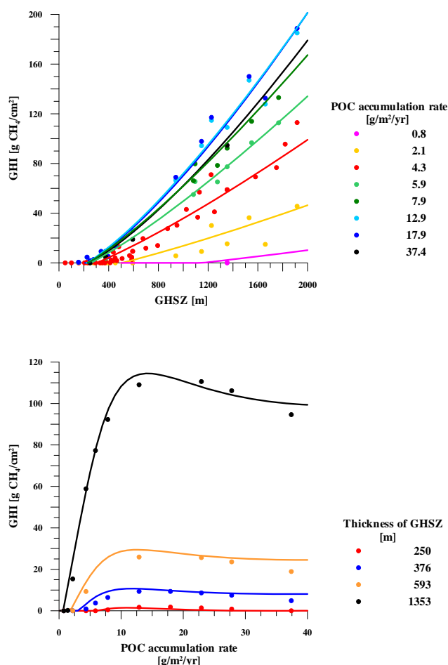
Fig. 11. Parameter analysis of the two key control parameters POCar and GHSZ: (a) relation of GHSZ and GH accumulation for varying POCar; (b) relation of POCar and GH accumulation for varying GHSZ.
