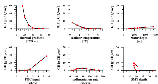
Fig. 9. Sensitivity analysis of the standard model: For each model run (red dots) only one input parameter was varied. Additionally, the output parameter SO_4 - CH_4 -transition depth (SMT) as a result of increasing the POCar is shown.
