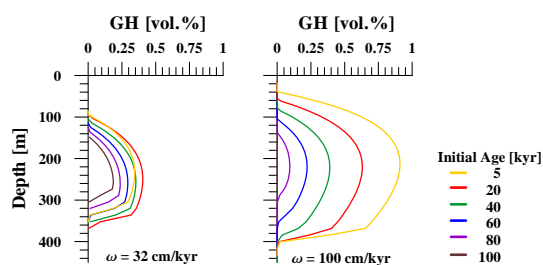
Fig. 8. Effect of the POC initial age ( age_{init} ) on the accumulation of gas hydrates in marine sediments at two different sedimentation rates ( \omega ).
