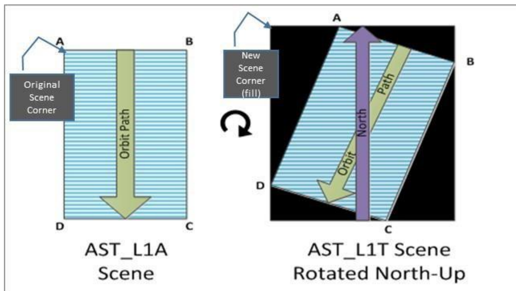
AST_L1A Image Rotated North-Up in AST_L1T Product
