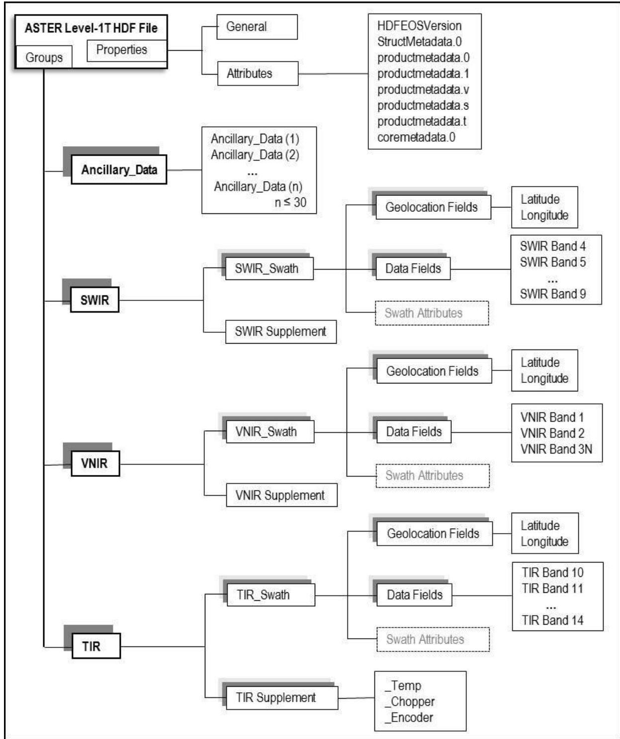
Figure 2.2-1. AST_L1T HDF File Structure
