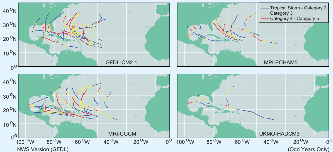
Simulated trajectory of hurricanes and tropical storms with A1B.
