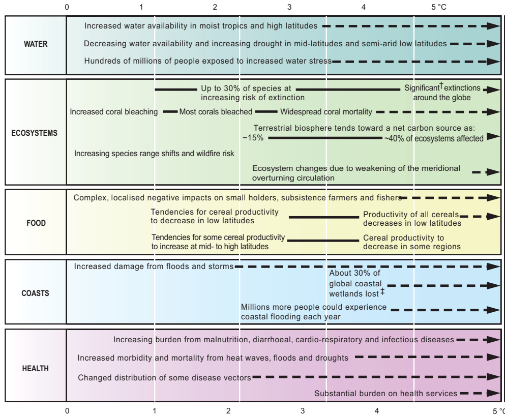
DIAGRAM I.1 POTENTIAL IMPACT OF GLOBAL AVERAGE ANNUAL TEMPERATURE CHANGE RELATIVE TO 1980 – 1999 (In degrees Celsius)
