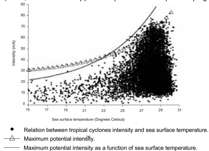
FIGURE 7.6 PACIFIC OCEAN: CYCLONES INTENSITY AND SEA SURFACE TEMPERATURE (Scatter diagram of events, measured in intensity per meters per second and temperature by degrees Celsius)
