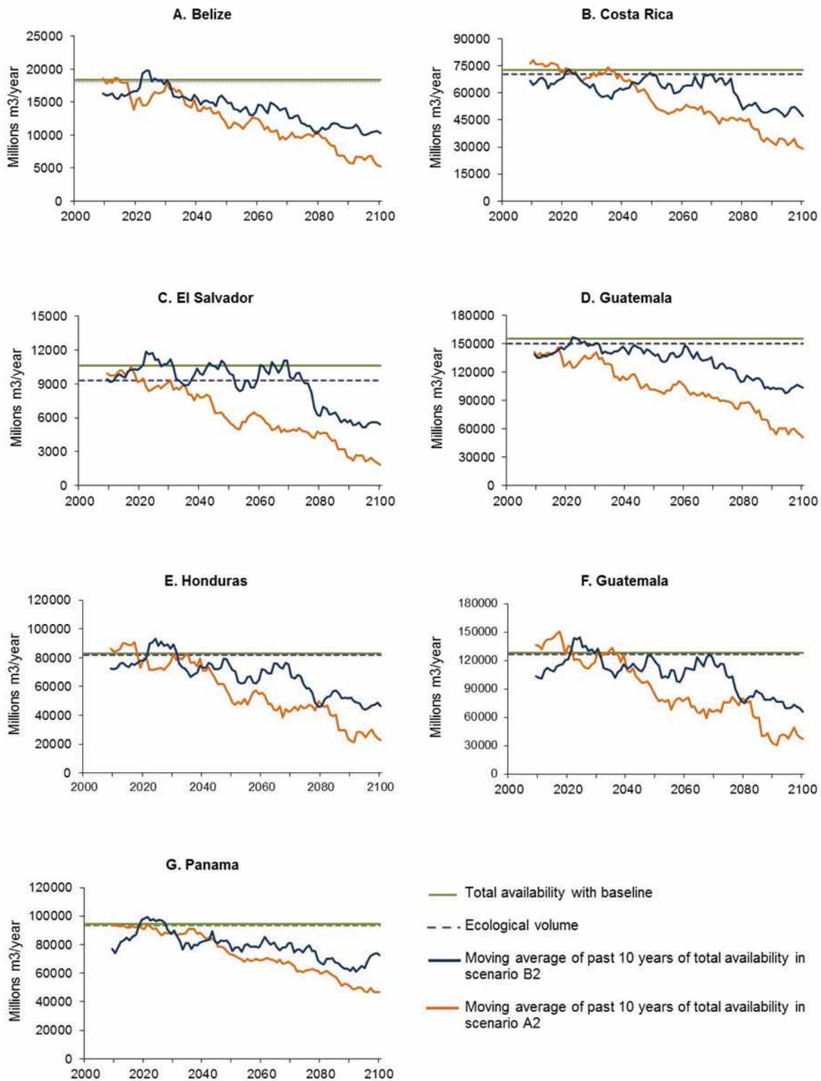
FIGURE 4.2 CENTRAL AMERICA: TOTAL AVAILABILITY OF RENEWABLE WATER, BASELINE SCENARIO, B2 AND A2, 2000-2004 TO 2100 (In millions of cubic meter per year with simple average of three models)
