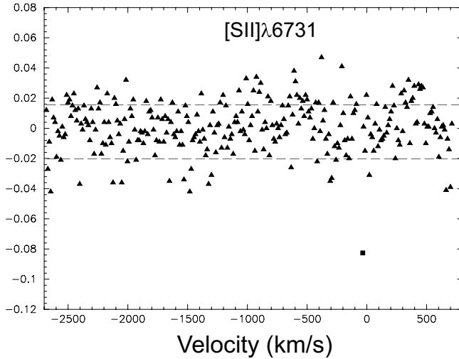
Figure showing the displacement in the [OI] \lambda 6300, 6363, HeI \lambda 6678 and [SII] \lambda 6731 emission line regions, with respect to the continuum measured across a large part of the individual orders. Note that at no other point in any of the lines do the significant displacements measured at the forbidden ELRs occur.
