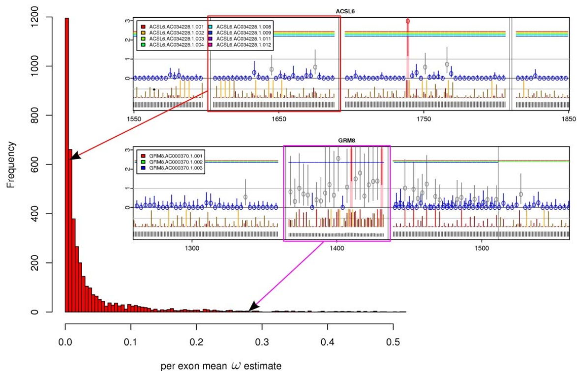
Supplementary Figure 5: Examples of sitewise \omega analyses. The upper panel is from the ACSL6 gene of ENCODE target region ENm002. At the top, the colored horizontal lines and legend indicate the exons that contribute to each proposed transcript variant (001, ... , 012). The color of sitewise \omega estimates (circles) and their confidence intervals (bars) denote the inferred mode of selection acting: blue: purifying selection; grey: unclassified; red: adaptive evolution (also highlighted with a pink background). Below this is a per-nucleotide measure of conservation, with abnormally fast sites colored orange (3rd codon positions) or red (1st or 2nd codon positions). The black bars at the bottom record the number of sequences available at each alignment position. The upper panel is typical of a good protein sequence alignment. The exon boxed in red has a typical exon-wide mean \omega , indicated by the arrow showing its position relative to the distribution of the means from the full data. Note the single site (position 1740) for which significant positive selection is inferred. The lower panel is from GRM8 (Enm014). The exon boxed in purple (only present in transcript variant 003) has an atypical mean \omega value, and comprises many sites inferred to have neutral or positively selected evolutionary dynamics. The preceding exon is not unusual; in the following one, variant 003 is in a different reading frame, terminates early and again has an unusual pattern of sitewise \omega estimates. This is suggestive that variant 003 is under unusual selective pressures or is not protein coding.
