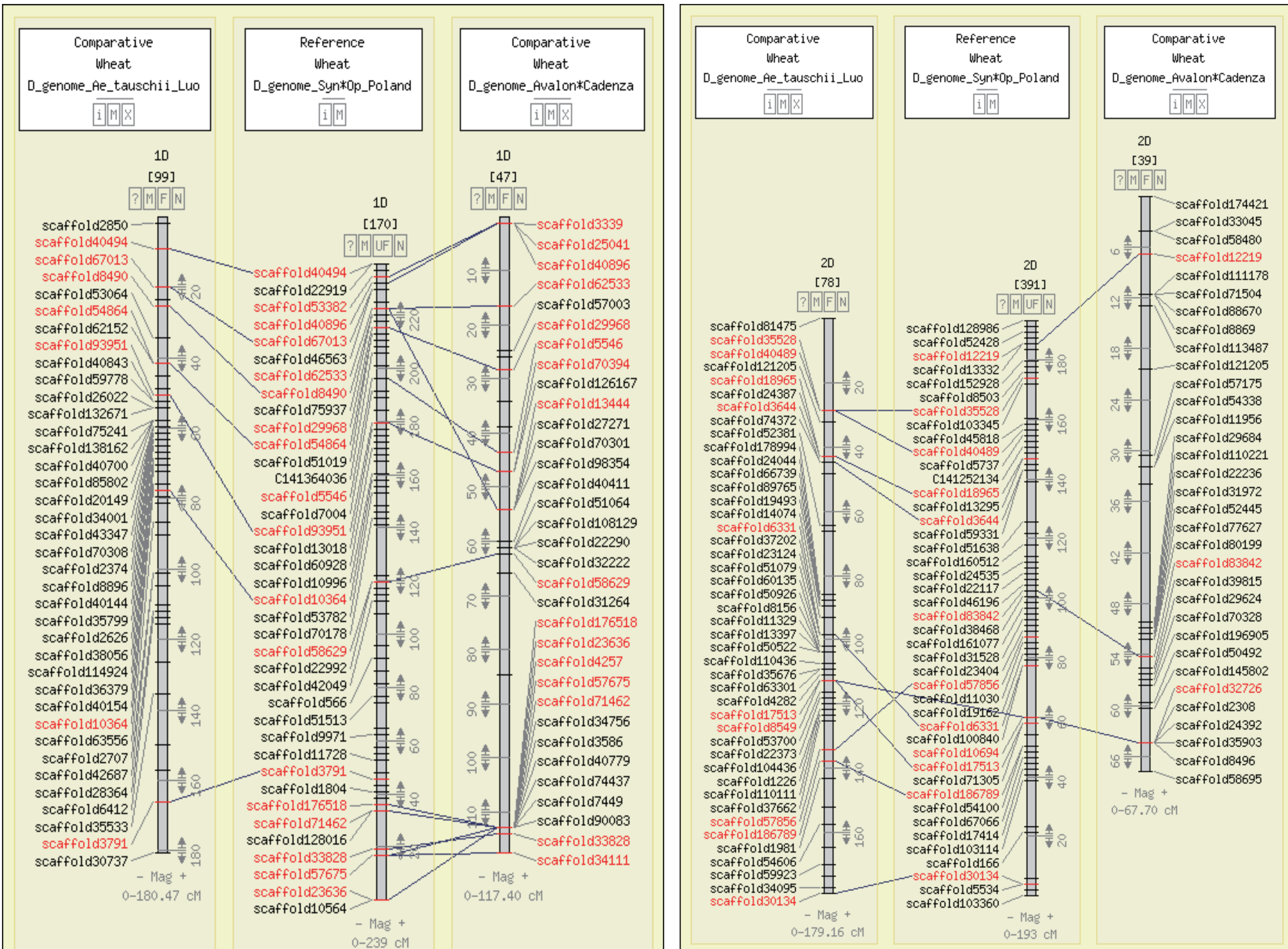
Supplementary Figure 15: CMap based comparisons of three SNP-based maps.
