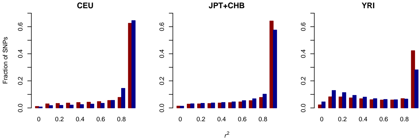
Figure S1: Fraction of SNPs in HapMap Phase II captured by r^2 of at least a given threshold by Illumina 300K (blue) and Affymetrix 500K (red).
