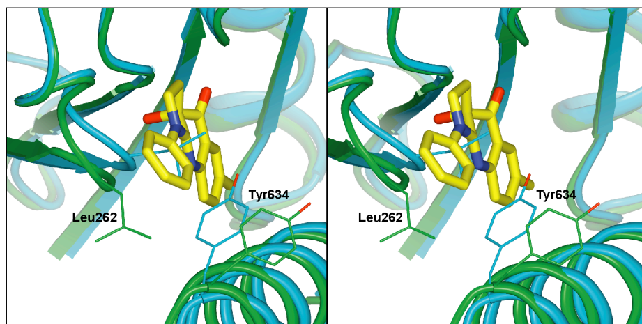
Supplementary Figure 2. Stereo view of the apo and blebbistatin-bound forms of MgADP.Vi-S1dC myosin. Apo MgADP.Vi-S1dC myosin (accession number 1VOM) is shown in blue while the blebbistatin-bound form is in green. Leucine 262 and Tyrosine 634 are shown as stick representations for both structures. Blebbistatin is shown as the yellow stick representation.
