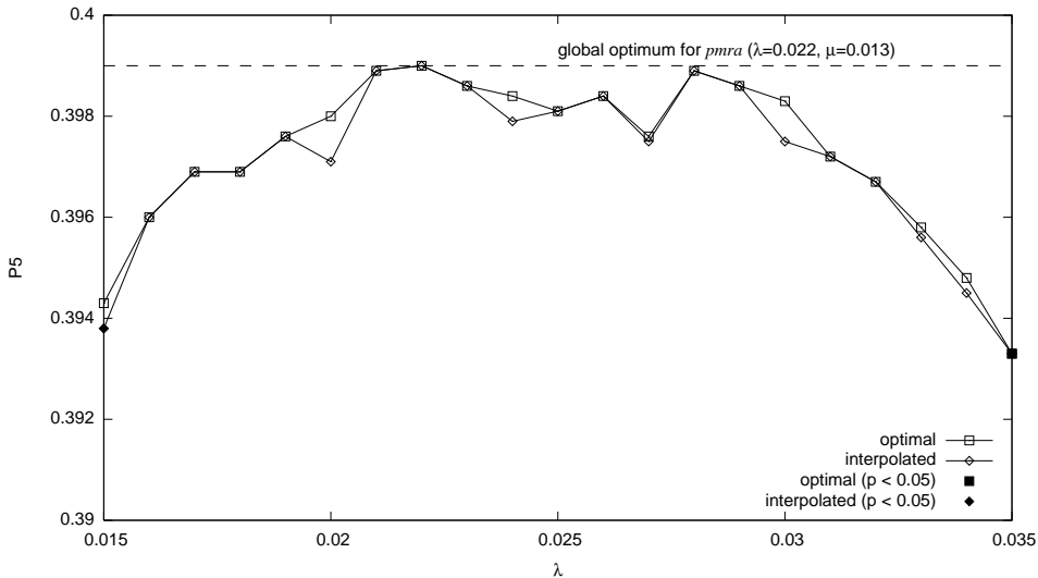
P5 at optimal and interpolated values of \mu for each \lambda in the pmra model
