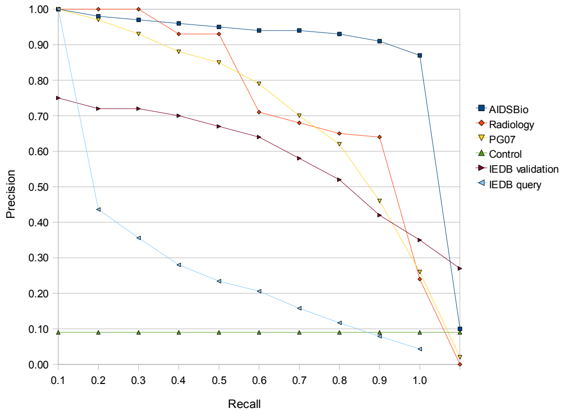
11-point interpolated precision curves
