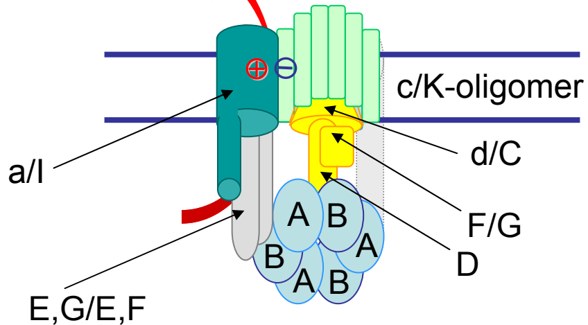
V-type ATPase
